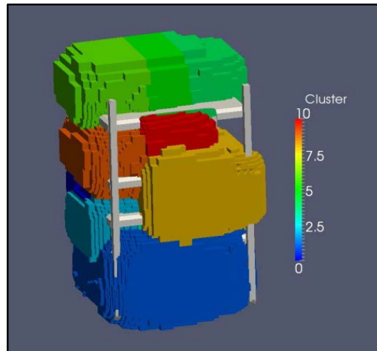
Figure 38: Clusters around equipment with the geometric distance calculated from their bounding boxes. The weights are the same as in the prior figure.
