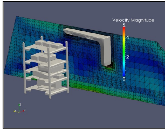
Figure 23: Typical vehicle HVAC mesh cutting plane.
