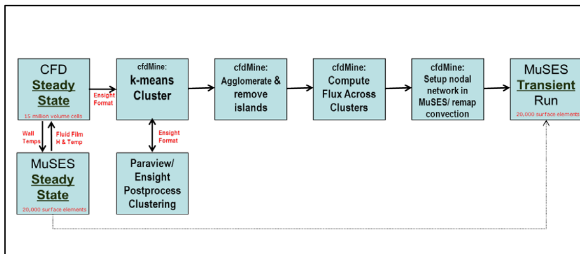
Figure 12: New process to use a steady-state CFD solution to create a transient MuSES thermal simulation.
