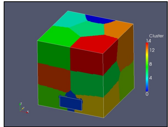
Figure 32: Clustering results for Case 1, clusters 0-14.
