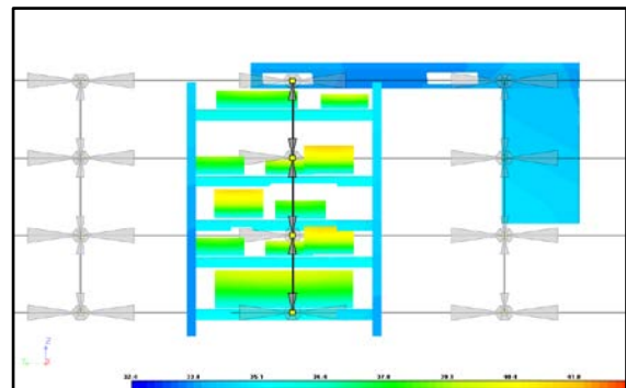
Figure 59: Close-up of the subvolume duct. Note the volumes cut complete across the shelves. Note there is multiple equipment associated with each node.
