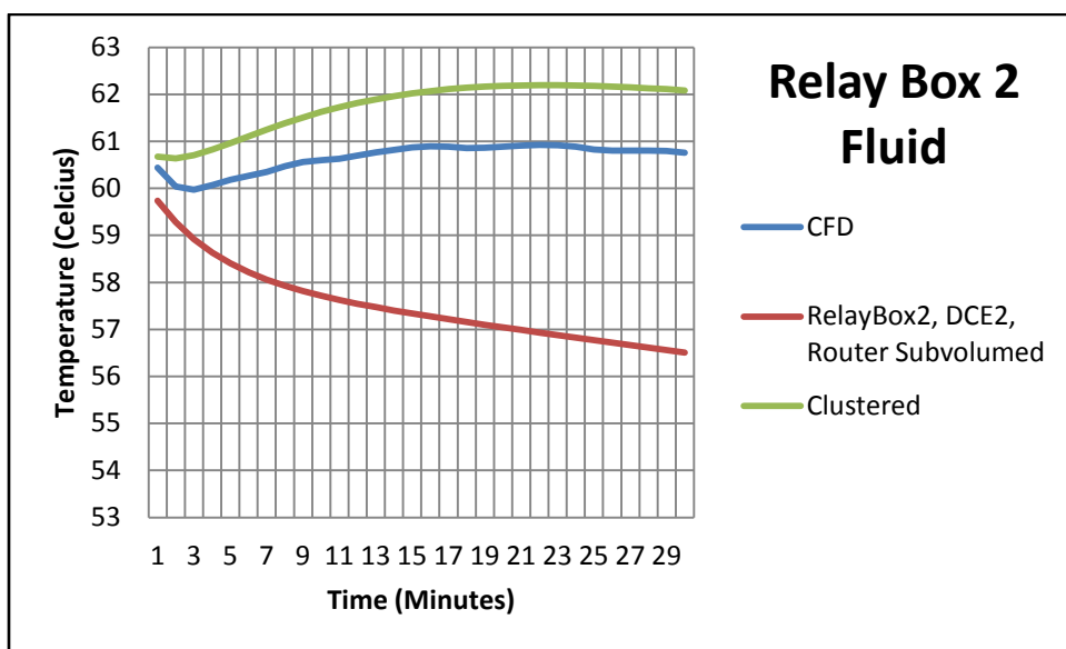
Figure 89: Relay Box 2 Fluid Temperature.
