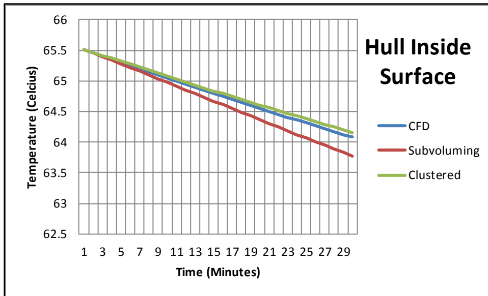
Figure 78: Hull Inside Surface Temperatures.
