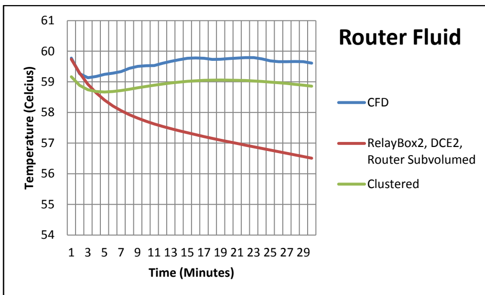
Figure 87: Router Fluid Temperature.
