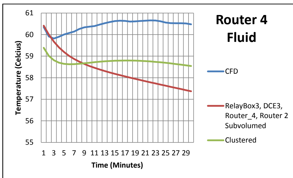
Figure 91: Router 4 Fluid Temperature.
