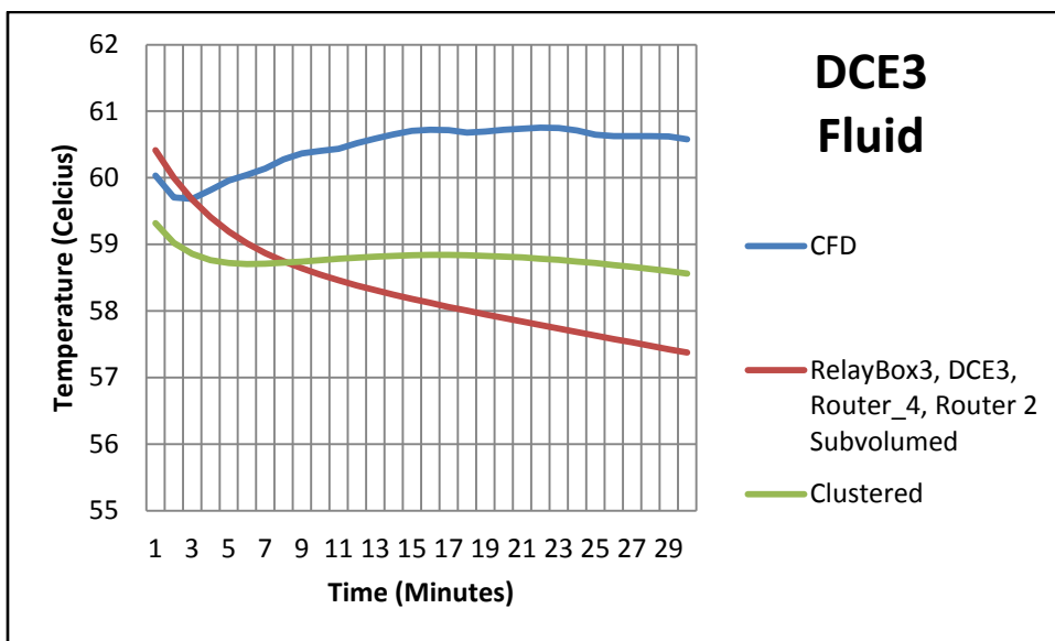
Figure 83: DCE 3 Fluid Temperature.
