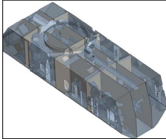
Figure 2: Example of decomposing a domain into a reduced-order network. Each box represents a lumped control volume and flow is tracked at the interfaces. Note the arbitrary break-up of the domain.
