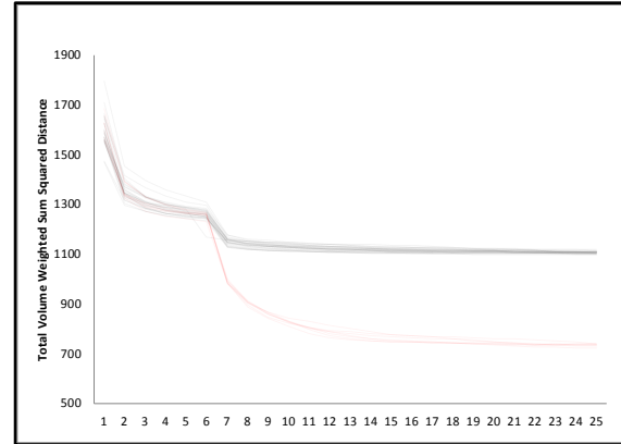
Figure 55: This is a "zoomed-in" plot of typical k-means convergence plot for 33 random start trials on a vehicle duct geometry. The lines are translucent. The black lines show 25 runs with a 50% Mahalanobis/Euclidean blend versus the 8 red lines which show 75% Mahalanobis. Note the first 5 iterations are pure Euclidean.
