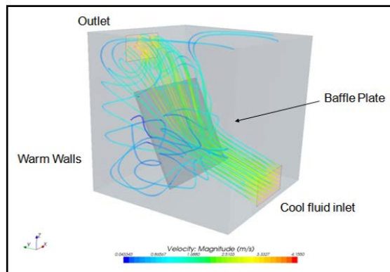
Figure 14: Test Case 2. This case consists of a cool fluid impinging on a baffle at a different angle and exiting from an outlet slot. The walls of the cube are held at a constant temperature. The mesh is 483162 volume elements.
