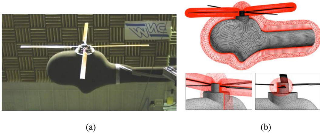
Figure 5: (a) HART-II rotor and test stand in the DNW wind tunnel, (b) Helios near-body meshes for HART-II rotor simulations.
