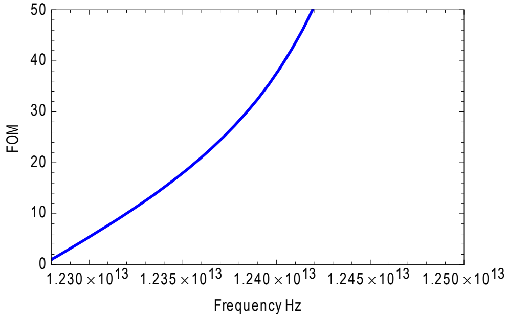
Fig. 6. Calculated figure of merit (FOM) as function of the frequency in Sn-Zn-doped indium oxide, all parameters are the same as in Figs. 3-4.
