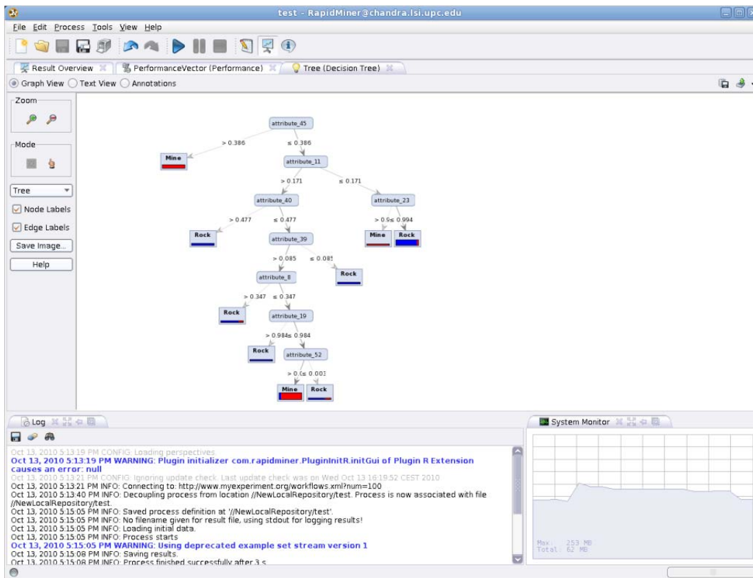
Figure 40 Result Perspective of RapidMiner: Decision Tree.
