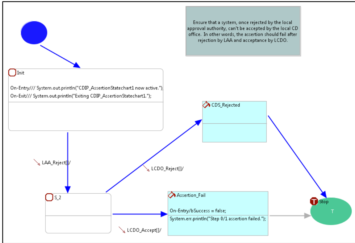
Figure 38. Statechart Assertion for Requirement R1
