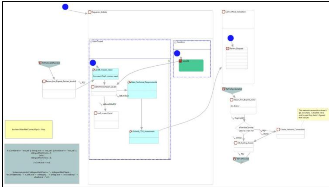
Figure 14. Sub-process Titled “Initiate_CDSR”
