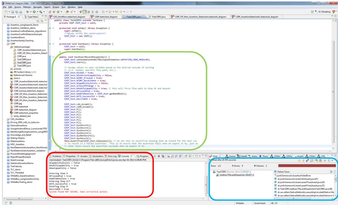
Figure 43. Manual Testing Example – Failed Assertion
