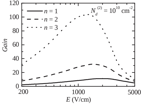
Fig. 22. Gain vs. electric field.
