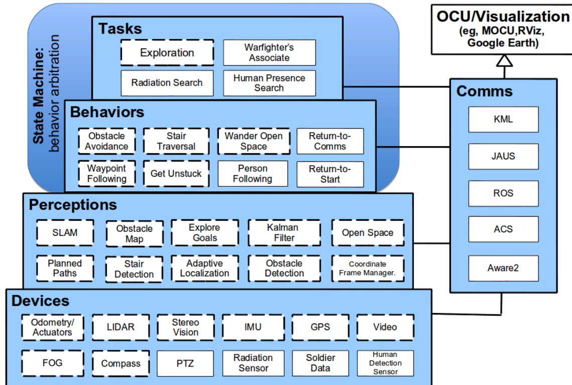
Figure 1: A simplistic illustration of the ACS module construct. Dotted boxes are example modules that are directly tied to the Exploration task described above.
