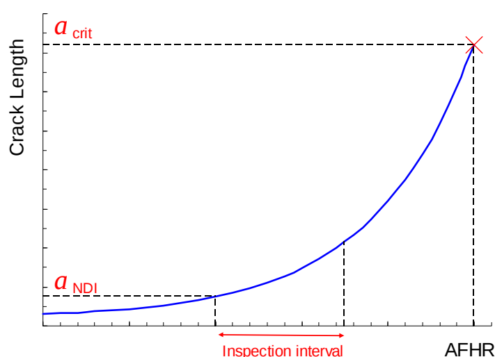
Figure 2 Inspection interval determined from a_{NDI} and crack growth curve (schematic)
