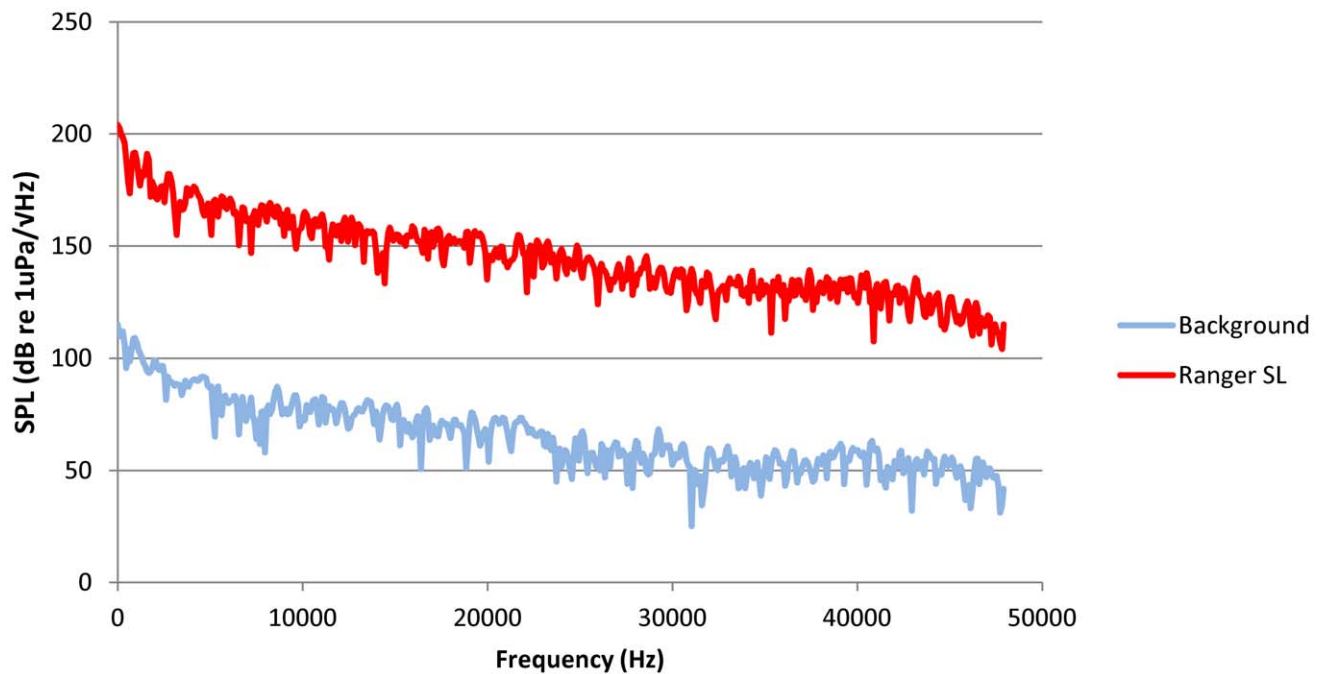
Figure 2. Predicted spectrum of source vessel noise expressed in units of power spectral density. The noise signature is dominated by low frequency noise ( <10 kHz) but has high levels across the frequency range of the recordings. doi:10.1371/journal.pone.0042535.g002
