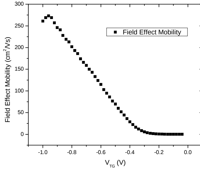
Figure 7: Field effect mobility (hole ) as a function of top gate Vgs. Note that the I_{ds} - V_{gs} plot was smoothed before the transconductance , g_m was calculated for field effect mobility assessment.
