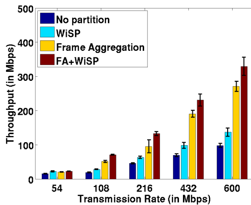
Figure 3.17: Performance comparison (with A-MPDU FA) for TCP flows at higher rates.
