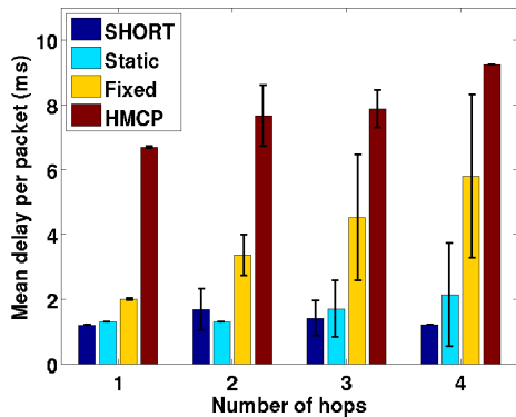
Figure 4.11: Average delay of VoIP packets sent with a TCP flow.
