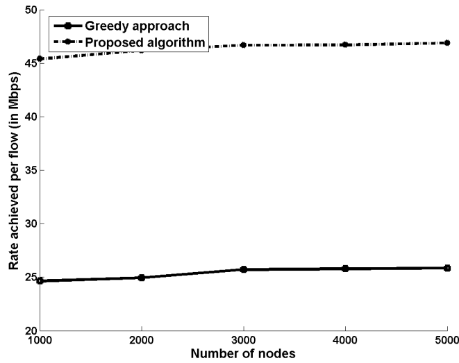
Figure A.5: Average rate achieved per flow as a function of network density.
