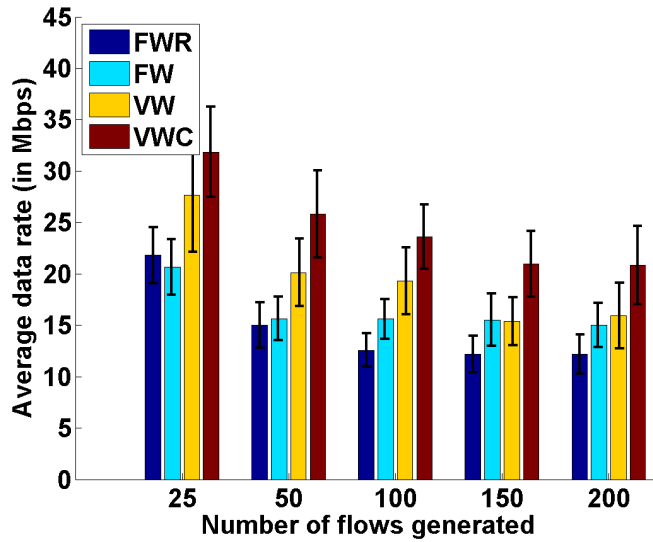
Figure 5.5: Average data rate of accepted flows.
