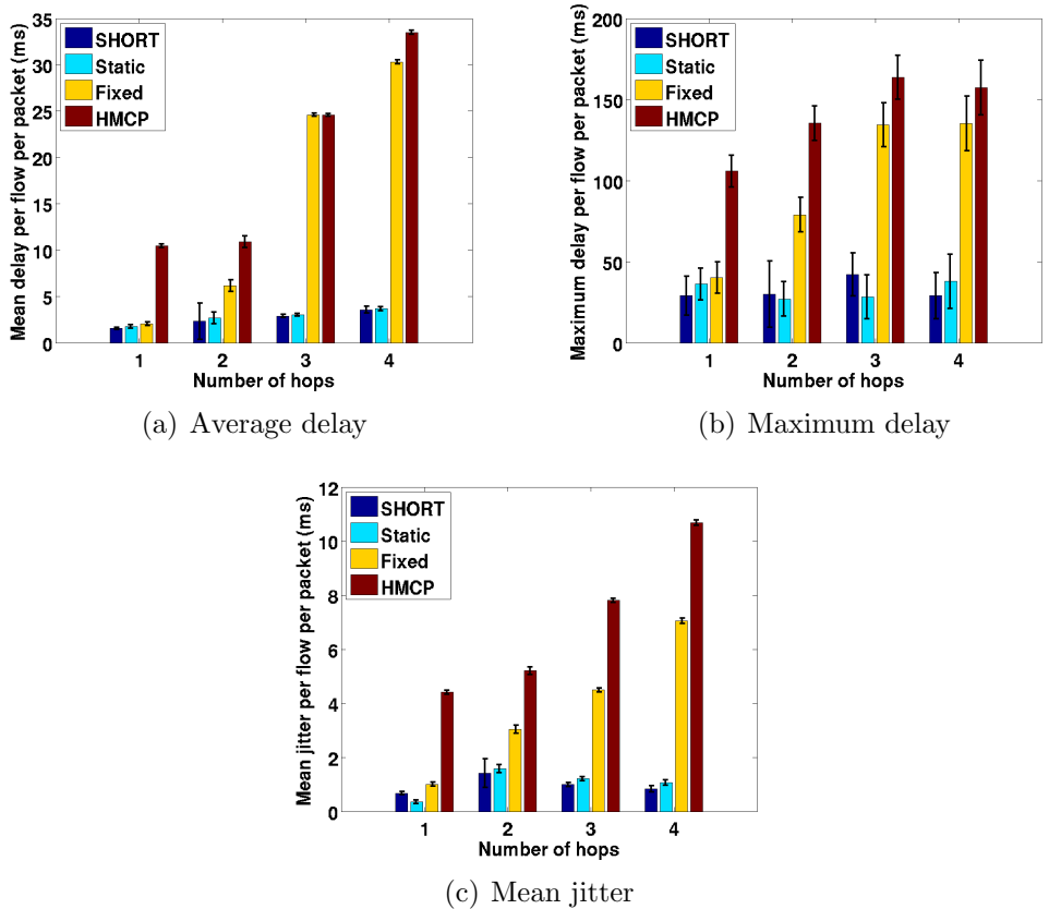
Figure 4.8: Performance comparison for multihop bidirectional VoIP flows.
