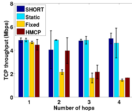
Figure 4.12: Throughput of TCP flow sent with a VoIP flow.
