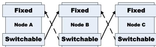
Figure 2.2: Example multi-channel protocol operation.
