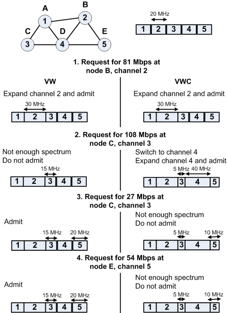
Figure 5.4: Illustration to compare number of accepted flows in VW and VWC.
