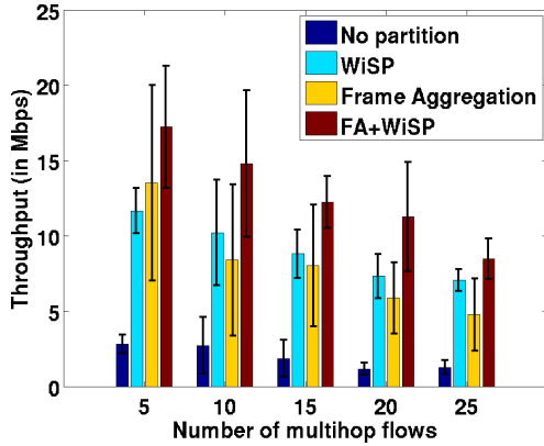
Figure 3.22: Performance comparison (with A-MPDU FA) of UDP flows over a single channel, multihop network.
