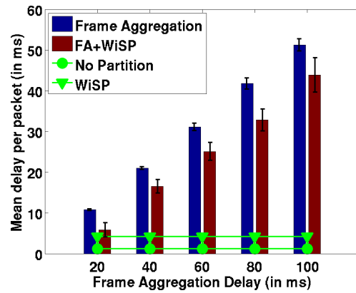
Figure 3.9: Mean packet delay comparison for TCP flows across various A-MSDU aggregation delays.
