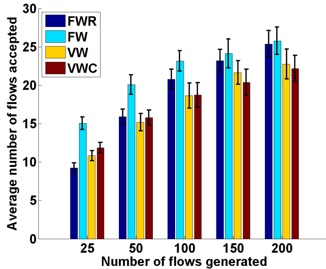
Figure 5.3: Average number of accepted flows.
