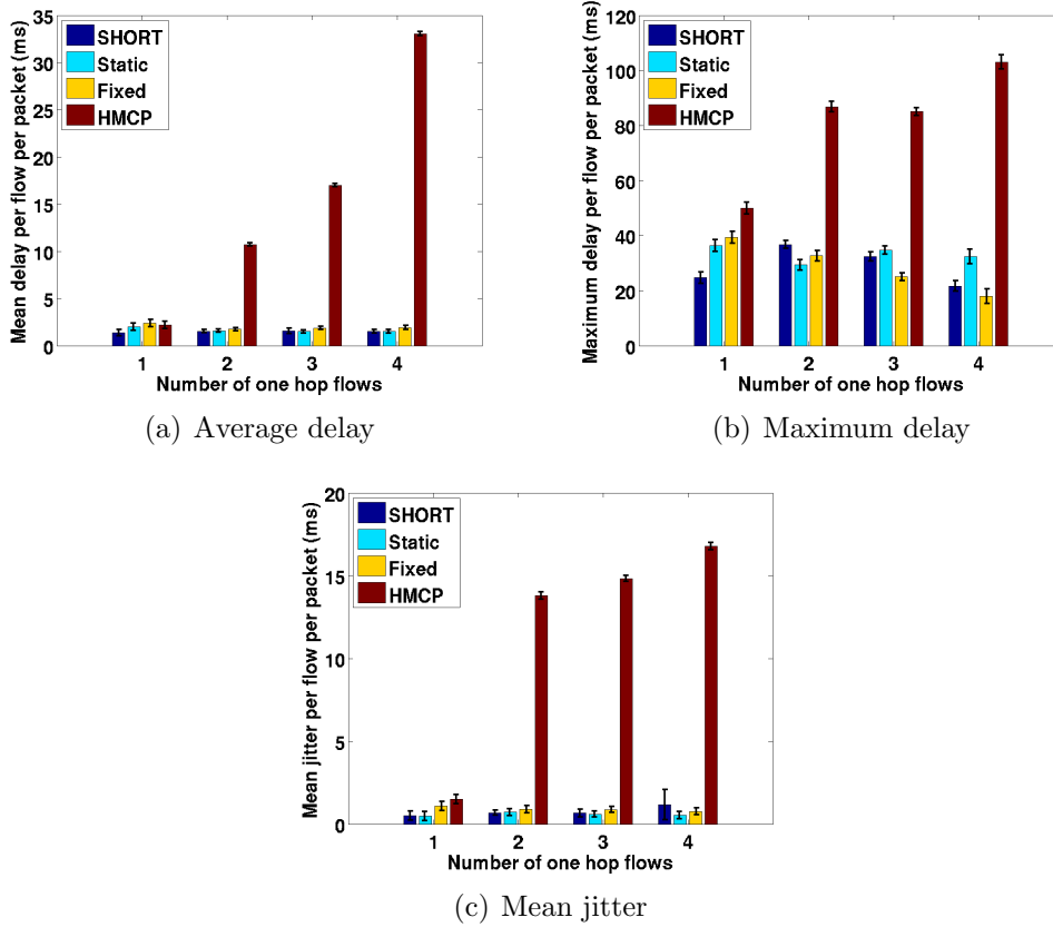
Figure 4.13: Performance comparison for multiple one hop VoIP flows from a node.
