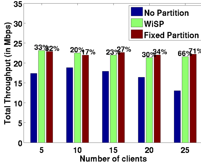
Figure 3.6: Performance of WiSP for TCP flows.
