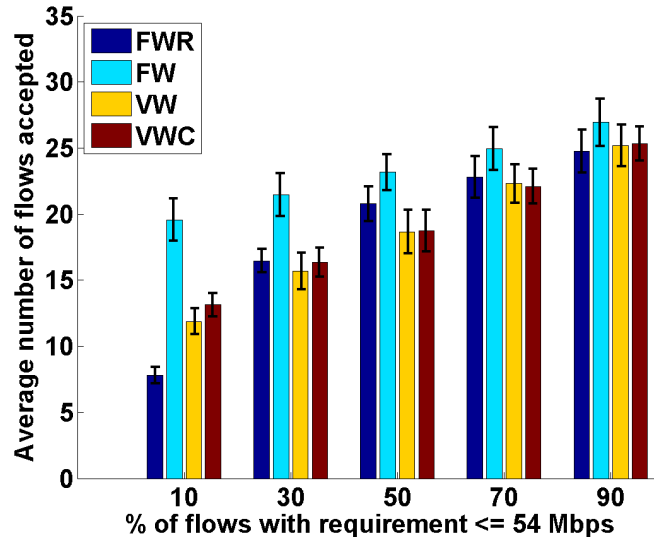
Figure 5.6: Average number of accepted flows with different percentage of low rate flows.
