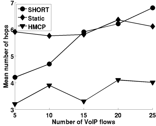
Figure 4.16: Number of hops taken by TCP flows.
