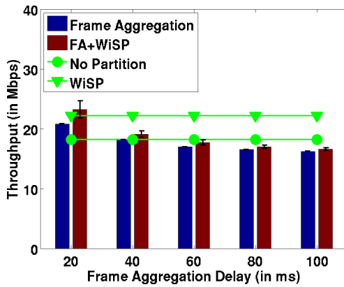
Figure 3.8: Throughput comparison for TCP flows across various A-MSDU aggregation delays.
