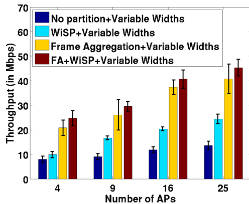
Figure 3.19: Performance comparison (with A-MPDU FA) for a multiple network scenario.
