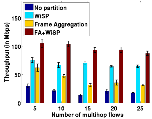
Figure 3.21: Performance comparison (with A-MPDU FA) of TCP flows over a multichannel, multihop network.
