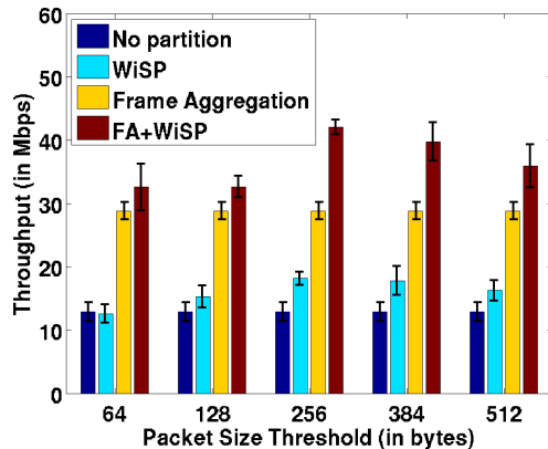
Figure 3.18: Performance comparison (with A-MPDU FA) across various packet size thresholds.
