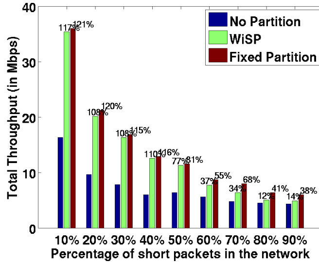
Figure 3.4: Validation of WiSP algorithm.
