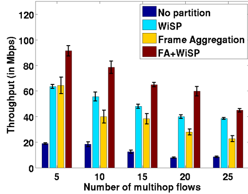
Figure 3.23: Performance comparison (with A-MPDU FA) of UDP flows over a multichannel, multihop network.
