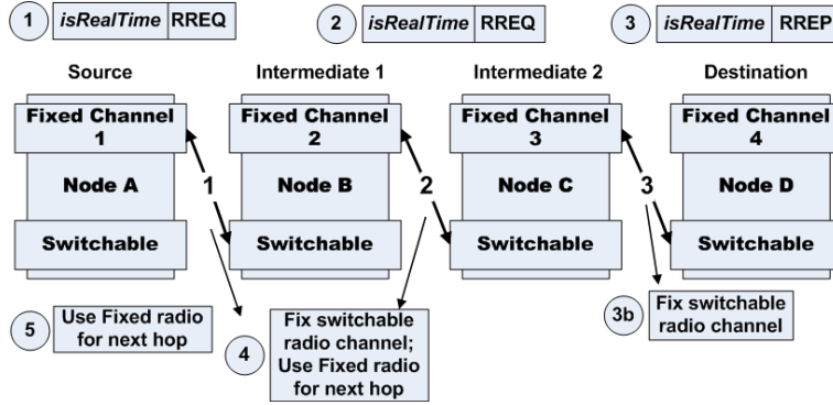
Figure 4.4: SHORT protocol steps.
