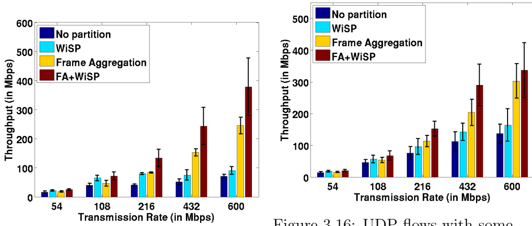
Figure 3.15: UDP flows with every client sending both short and long packets (with A-MPDU FA).
