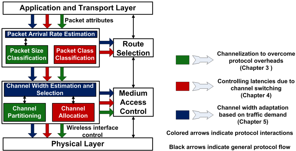
Figure 2.1: System Architecture.
