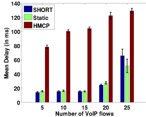
Figure 4.15: Delay comparison with more VoIP flows in a 100 node network.
