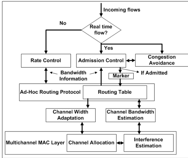
Figure A.1: Proposed protocol architecture.
