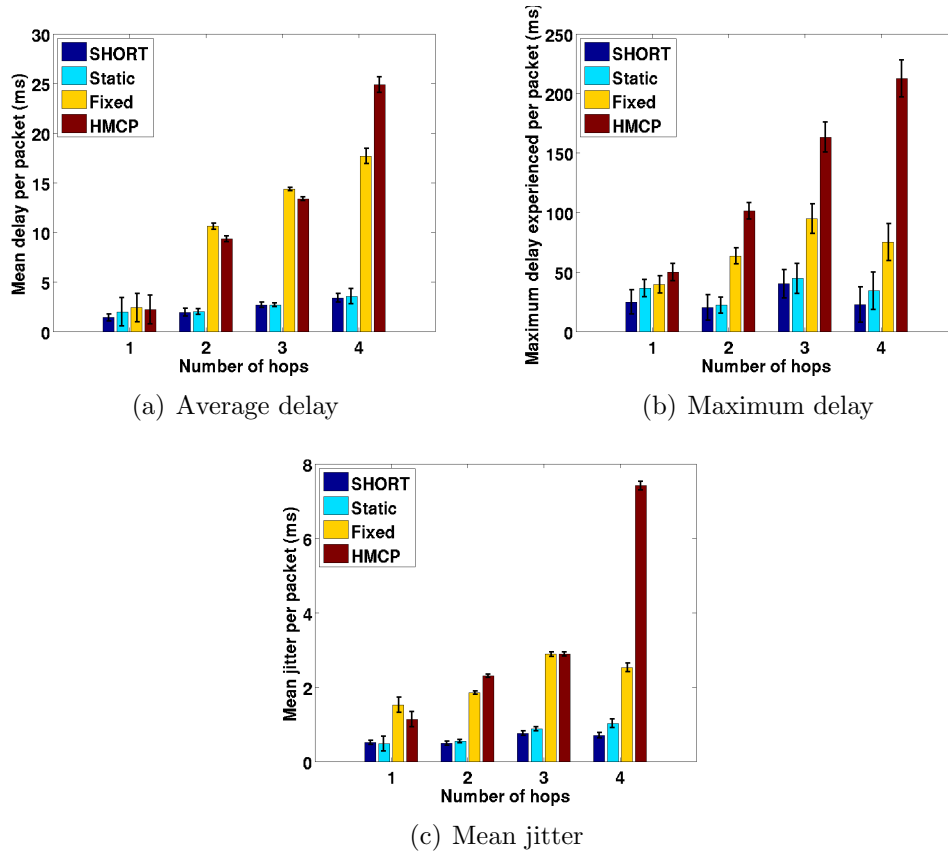
Figure 4.7: Performance comparison for multihop unidirectional VoIP flows.
