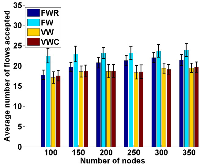
Figure 5.8: Average number of accepted flows with different number of nodes.
