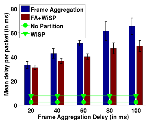
Figure 3.11: Mean packet delay comparison for UDP flows across various A-MSDU aggregation delays.
