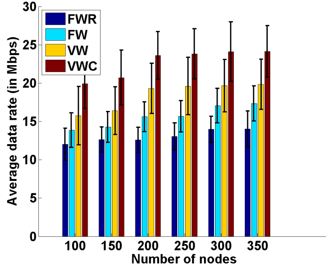
Figure 5.9: Average data rate of accepted flows with different number of nodes.
