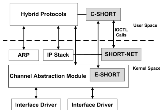
Figure 4.5: Protocol architecture with SHORT-specific components in gray.
