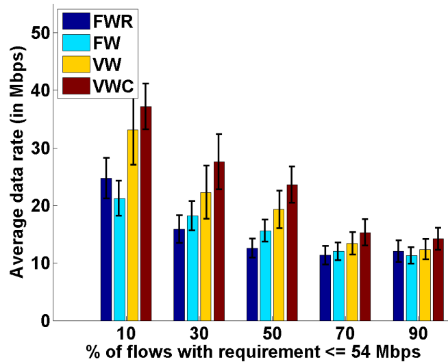
Figure 5.7: Average data rate of accepted flows with different percentage of low rate flows.
