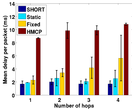
Figure 4.9: Average delay of VoIP packets sent with a UDP flow.
