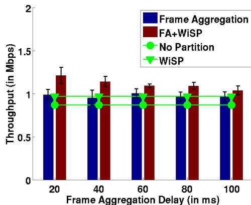
Figure 3.10: Throughput comparison for UDP flows across various A-MSDU aggregation delays.
