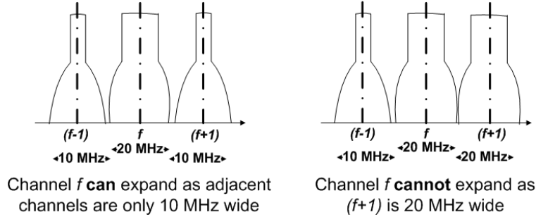
Figure 5.2: An illustration of allowed and disallowed channel width expansions. A check mark indicates that the expansion is allowed and a cross mark indicates that it is disallowed. (Figure not drawn to scale.)
