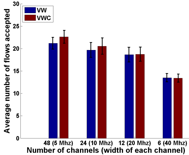
Figure 5.10: Average number of accepted flows with different number of channels.
