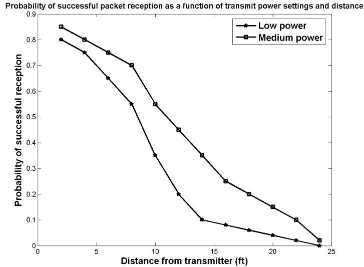
Figure A.2: Probability of successful packet reception as a function of distance and power.
