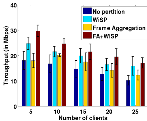
Figure 3.12: Performance comparison (with A-MPDU FA) for UDP flows with every client sending both short and long packets.
