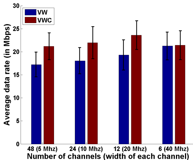
Figure 5.11: Average data rate of accepted flows with different number of channels.
