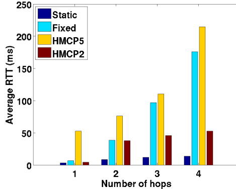
Figure 4.2: Results for pinging the nodes in flooding mode.
