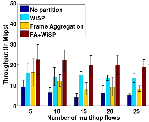
Figure 3.20: Performance comparison (with A-MPDU FA) of TCP flows over a single channel, multihop network.
