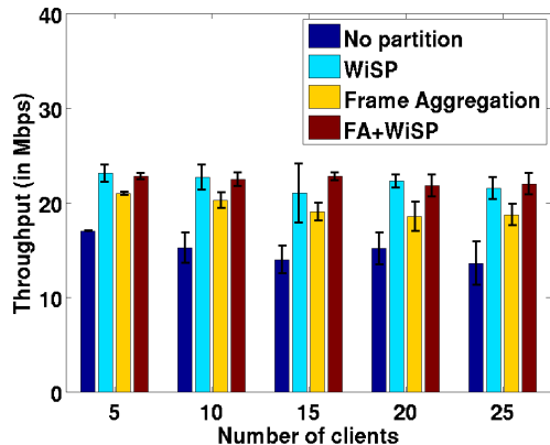
Figure 3.14: Performance comparison (with A-MPDU FA) for TCP flows.
