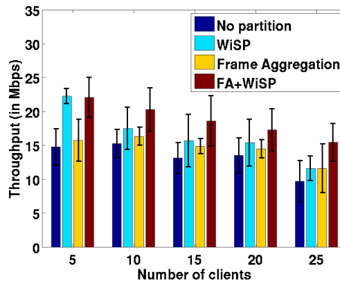
Figure 3.13: Performance comparison (with A-MPDU FA) for UDP flows with some clients sending only short packets and the rest sending only long packets.
