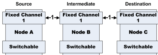
Figure 4.6: Fixed mode operation.
