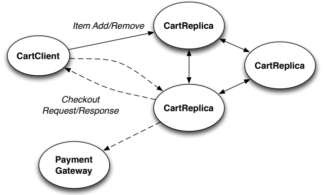
Figure 9: Shopping cart system architecture.
