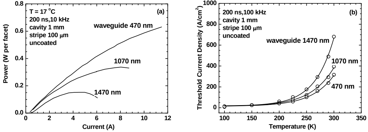
Figure 2. (a) Pulsed (200 ns, 10 kHz) light-current characteristics and (b) Temperature dependence of the threshold current density for 1-mm-long, 100- \mu\text{m} -wide, uncoated 3\ \mu\text{m} lasers having different waveguide widths.
