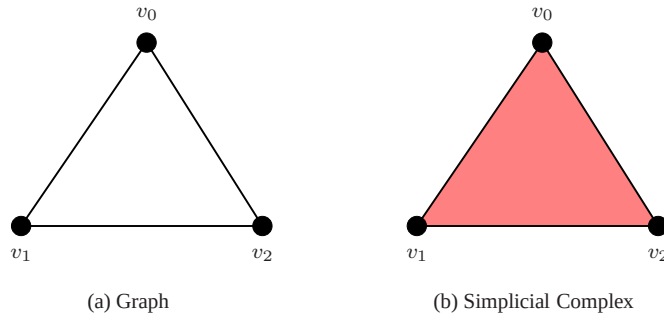
Fig. 1 Graph and simplicial complex: V = \{v_0, v_1, v_2\} , \mathcal{S}_{(a)} = \{(v_0, v_1), (v_0, v_2), (v_1, v_2)\} , \mathcal{S}_{(b)} = \{(v_0, v_1, v_2), (v_0, v_1), (v_0, v_2), (v_1, v_2), (v_0), (v_1), (v_2)\} .
