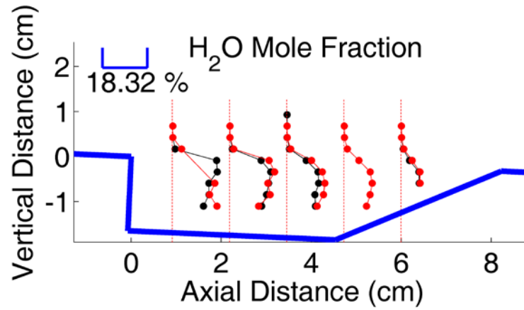
Fig. 16. Time averaged water mole fraction for no secondary air (black dots) and secondary air (red dots).
