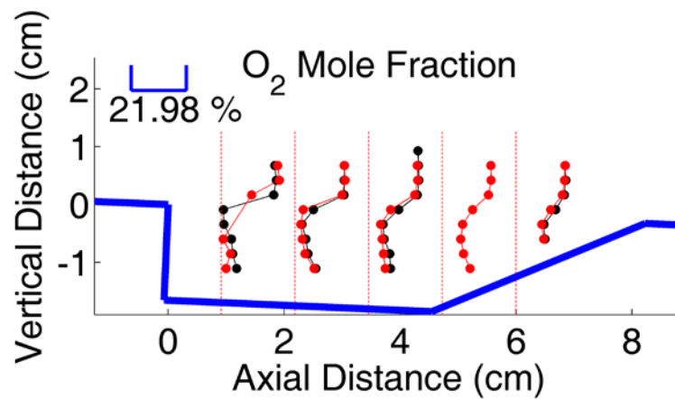
Fig. 17. Time averaged oxygen mole fraction for no secondary air (black dots) and secondary air (red dots).
