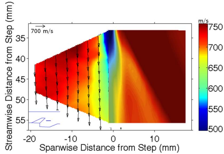
Fig. 4. Side-by-side comparison of 300 shot experimental (left) and LES predictions (right) of streamwise average velocity at y = 12.7 mm for the strut configuration. The LES predictions are at the same location as the experimental data and subsequently flipped across the centerline for direct comparison. Arrows in the experimental data indicate the 2D velocity.
