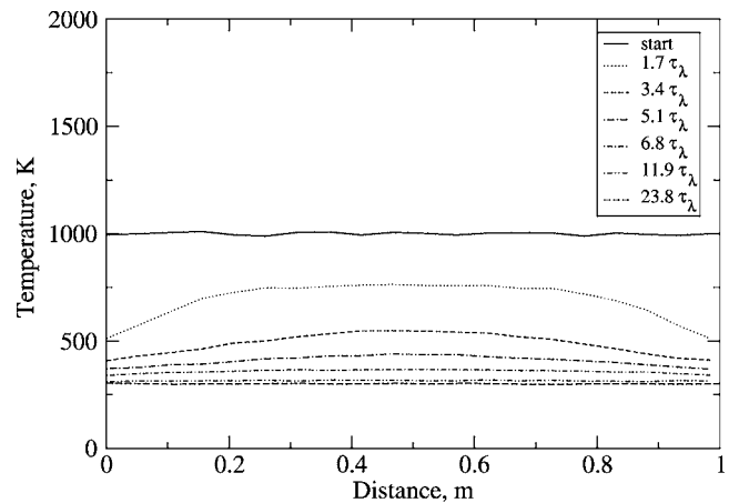
FIG. 3. Thermal relaxation of helium in a 300 K box. Time is in mean collision times, \tau_\lambda , at 1000 K.
