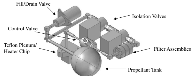
Fig. 3 Technology-demonstration FMMR (flight version).
