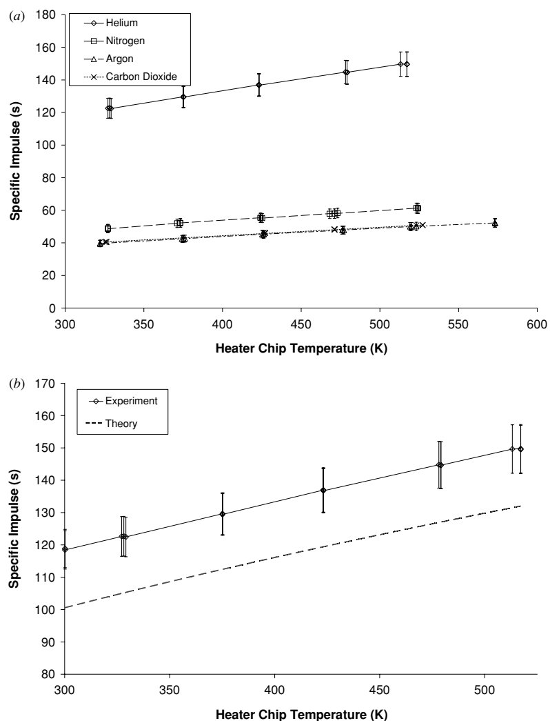
Figure 14. Specific impulse versus heater chip temperature for (a) various propellants. (b) Helium compared with free molecule theory.
