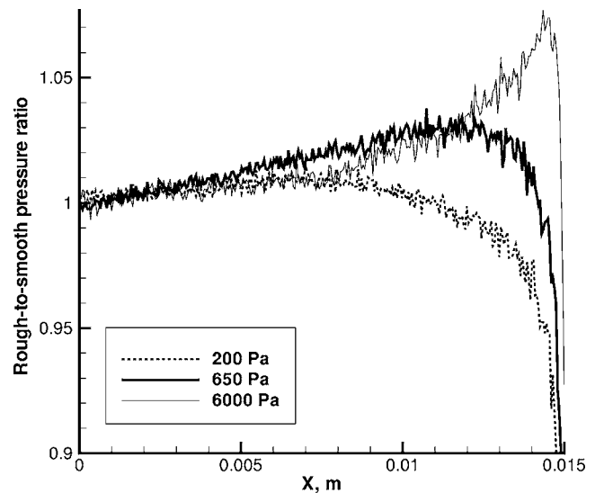
FIG. 10. Pressure ratio as a function of distance downstream along the centerline, conical rough surface to the smooth surface.
