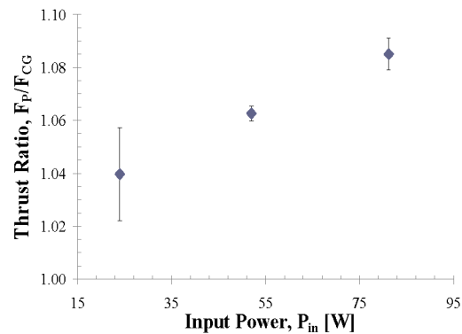
FIGURE 7. Thrust ratio as a function of input power.
