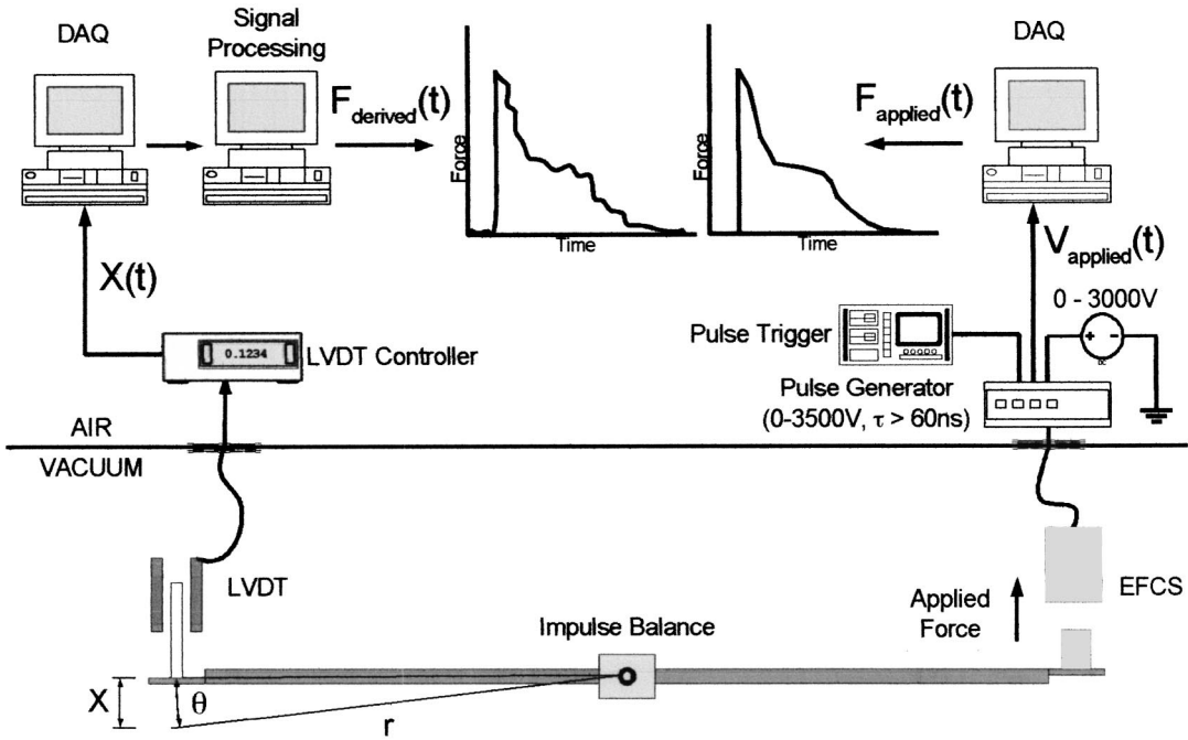
FIG. 6. Schematic of NIBS experimental setup and TRIM process for obtaining the derived and applied forces imparted to the impulse balance as a function of time.
