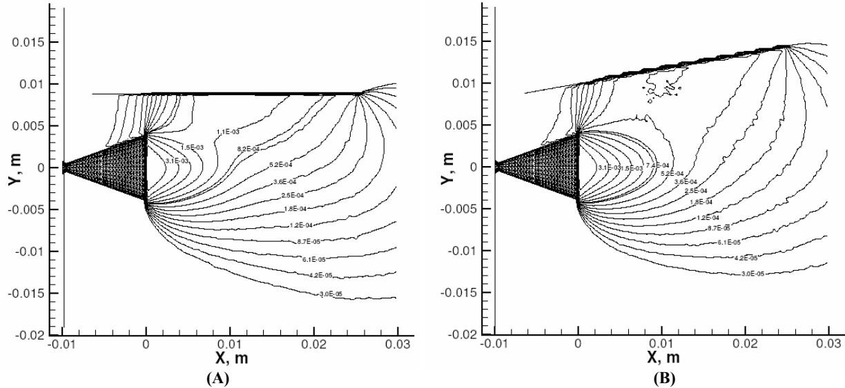
FIGURE 5. Pressure profiles for \text{Re}=270 nitrogen flow. (A) \alpha=0^\circ , (B) \alpha=10^\circ .
