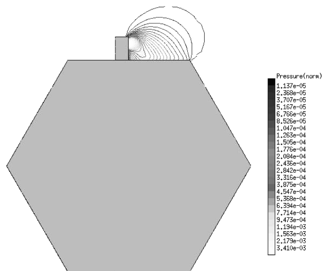
Fig. 17 Normalized pressure field for P_0 = 306.5 Pa and T_w = 573 K.
