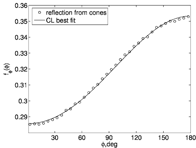
FIG. 2. Distribution function of the angle between the reflected tangential velocity and the flow direction, M=0.3 , \beta=66^\circ .
