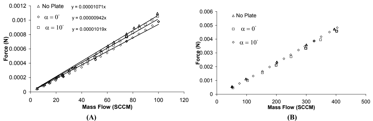
FIGURE 3. Thrust versus mass flow for nitrogen propellant. Measurements for free expansion, and engineering surface at \alpha=0^\circ and 10^\circ (A) Mass flow from 0 to 100 SCCM, (B) Mass flow from 50 to 400 SCCM.
