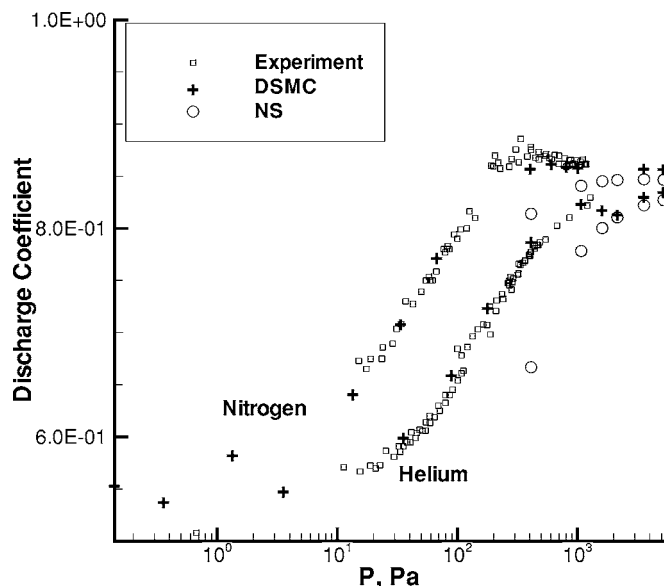
FIG. 5. Discharge coefficient versus plenum pressure for helium and nitrogen at t/d=0.015 : numerical modeling and experiment.
