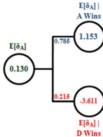
Figure 16 - Utility Function
