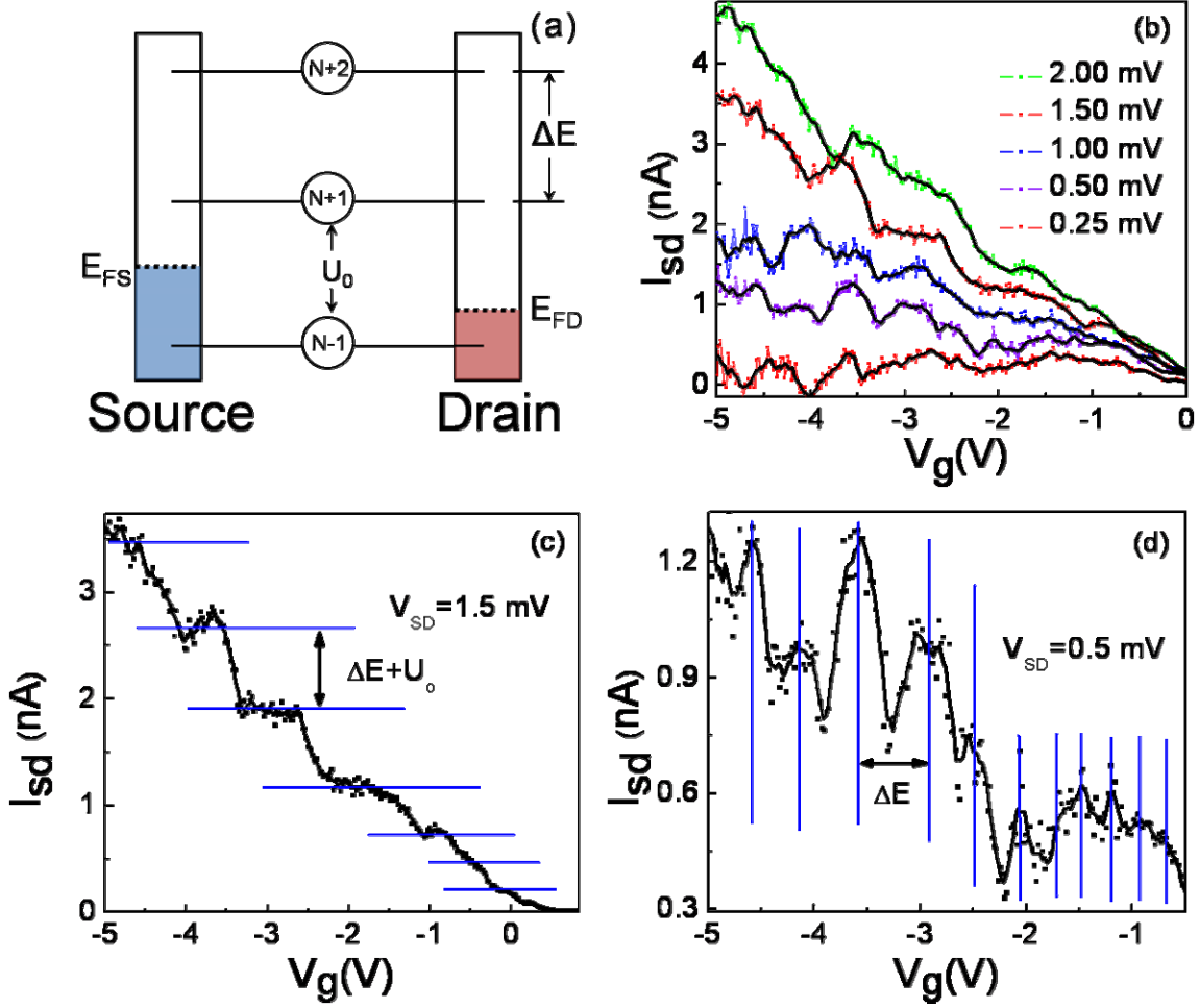
Figure 8: Characterization of SET performance. (a) Energy diagram for Coulomb blockade illustrating the transport window ( E_{FS} - E_{FD} ), the QD energy spacing \Delta E and potential energy U_0 which increases for each additional loaded electron. (b) I_{sd} versus V_g sweeps showing Coulomb oscillations which vanish at higher V_{sd} bias. (c) and (d) highlight two traces taken at V_{sd} = 1.5 mV (c) and V_{sd} = 0.5 mV (d). All measurements are carried out at 5.2K.
