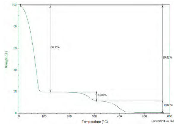
Figure 8. HC-CH-750 Dispersion TGA
