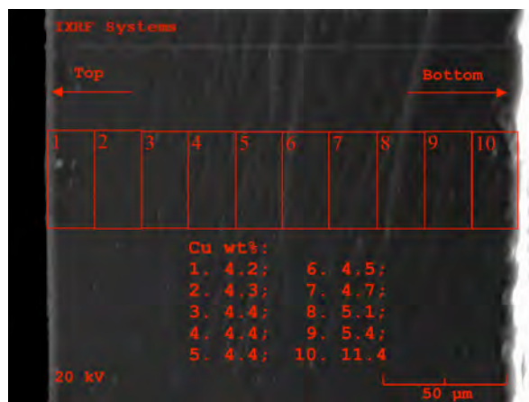
Figure 22. SEM cross-section of nanocopper-nanolatex film derived from 1% w/w copper suspension. The red superimposed grid illustrates how an EDAX analysis was done for measuring Cu concentration across the film. The righthand boundary is the film bottom, and there you can see some evidence of nanoparticle sedimentation.
