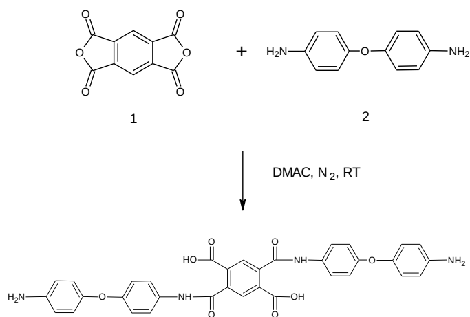
Figure 54. Polyamic acid synthetic pathway.
