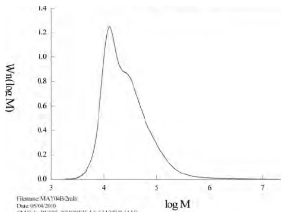
Figure 7. Absolute molecular weight distribution determined by light scattering detection of triblock 09-1049-28.
