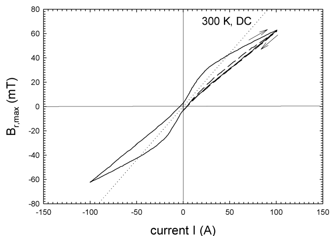
Fig. 4. Maximal values of the radial field component B_{r,\text{max}} ( r = 15 \text{ mm} ) as a function of DC current: at room temperature (dotted line), at 77 K and a half cycle 0 \rightarrow 100 \text{ A} \rightarrow 0 (dashed line) and at 77 K and the full cycle 0 \rightarrow 100 \text{ A} \rightarrow 0 \rightarrow -100 \text{ A} \rightarrow 0 (full lines).
