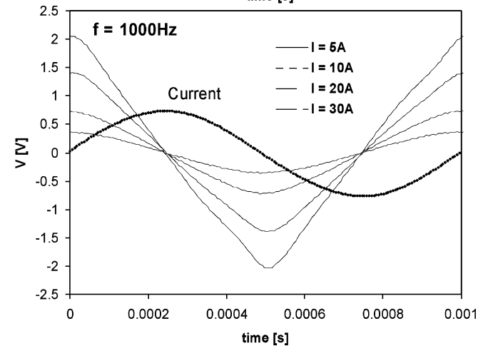
Fig. 8. Coil voltage V vs. time t , measured at 500 Hz and 1000 Hz at various current (rms values).
