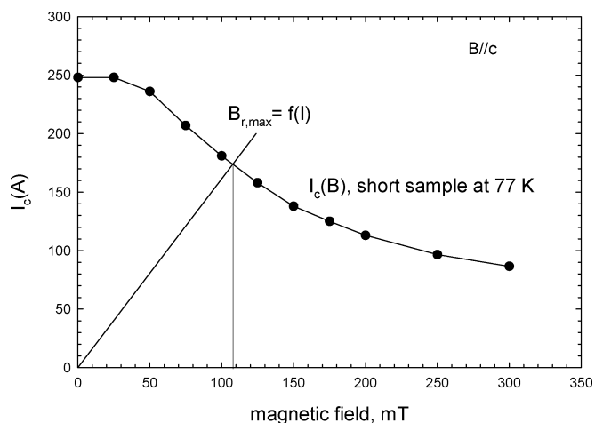
Fig. 5. The load line B_{r,\text{max}}(I) and I_c(B) curve of the YBCO tape used in the coil.
