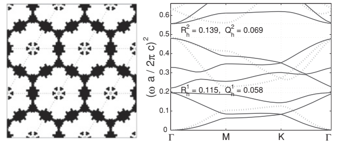
FIG. 8. Optimization results for the multiple complete band gaps in the hexagonal lattice. The optimal crystal structure is shown in the left-hand picture; while the frequency bands are shown in the right-hand picture, with solid lines representing TM bands, and broken lines representing TE bands. The first complete band gap is formed by the overlapping of the first TE and third TM band gaps, while the second complete band gap is formed by the third TE and sixth TM band gaps.
