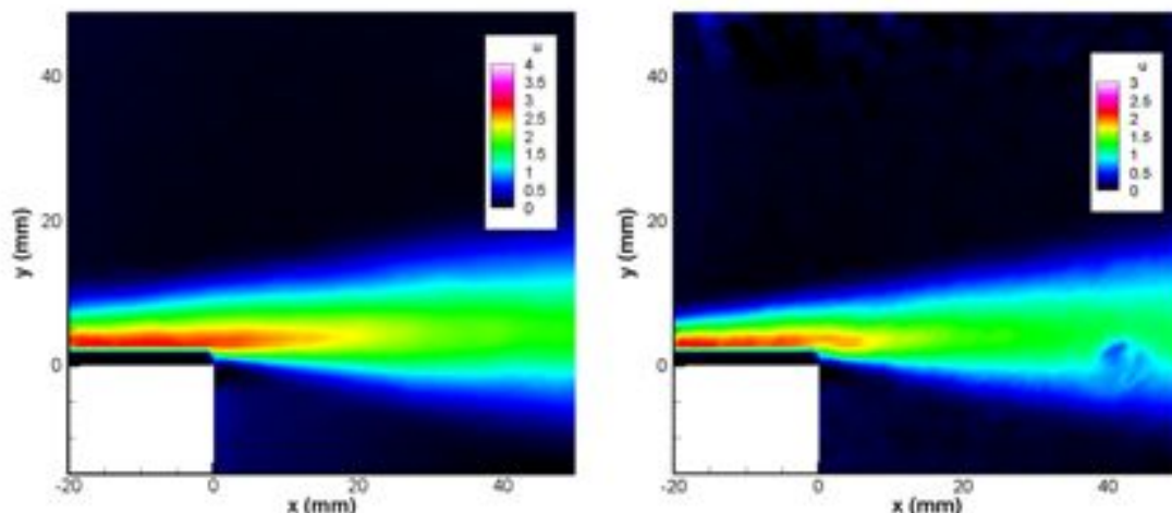
Figure 72 – Flow fields for 2 actuators (left) and 4 actuators (right) at 16kVpp.
