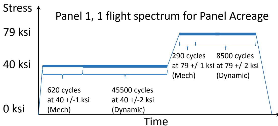
Figure 7.1.1 Single Flight Spectrum for Panel 1 Acrease
