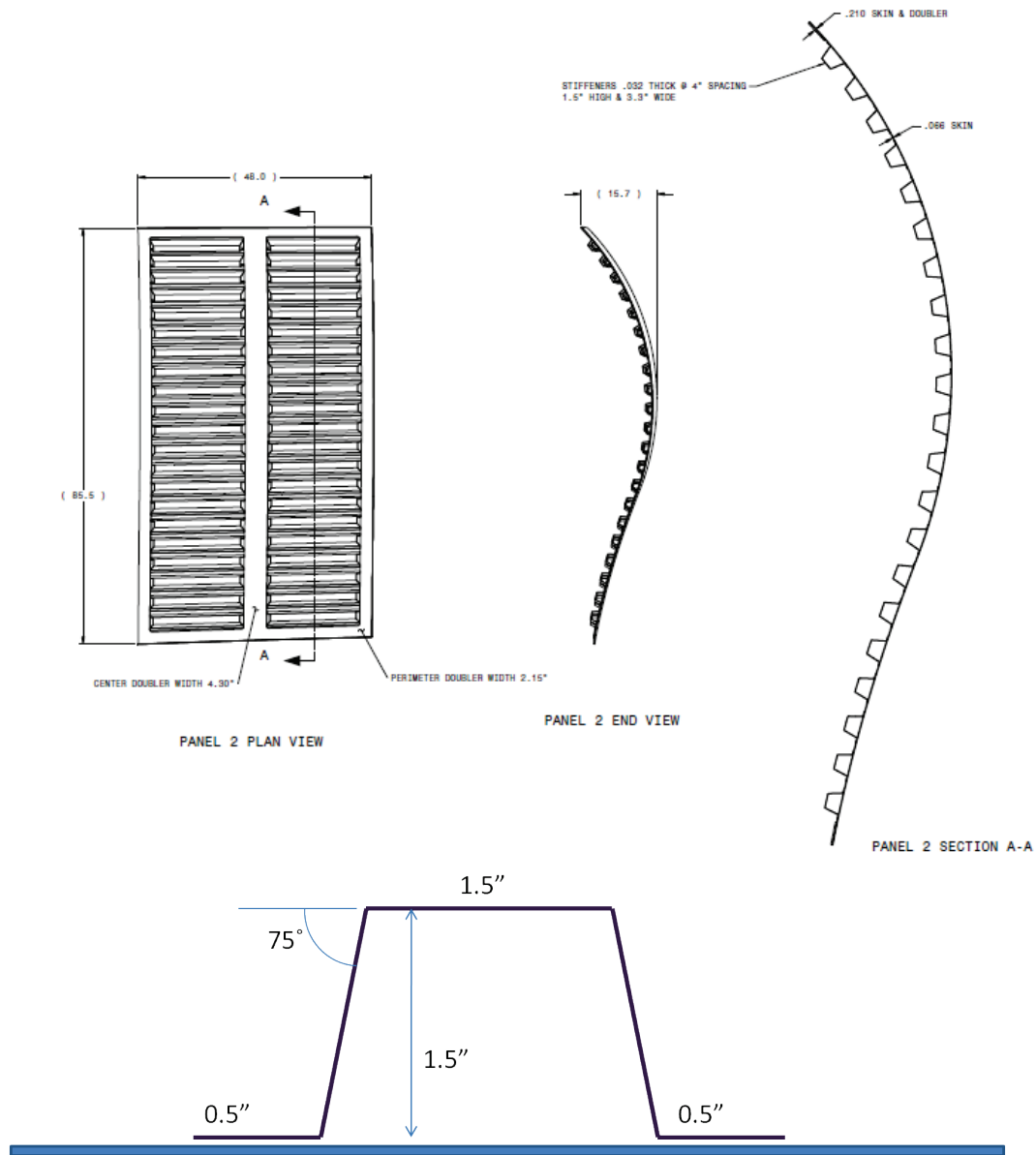
Figure 8.2.1 Panel 2 Dimensions and Hat Stiffener Details
