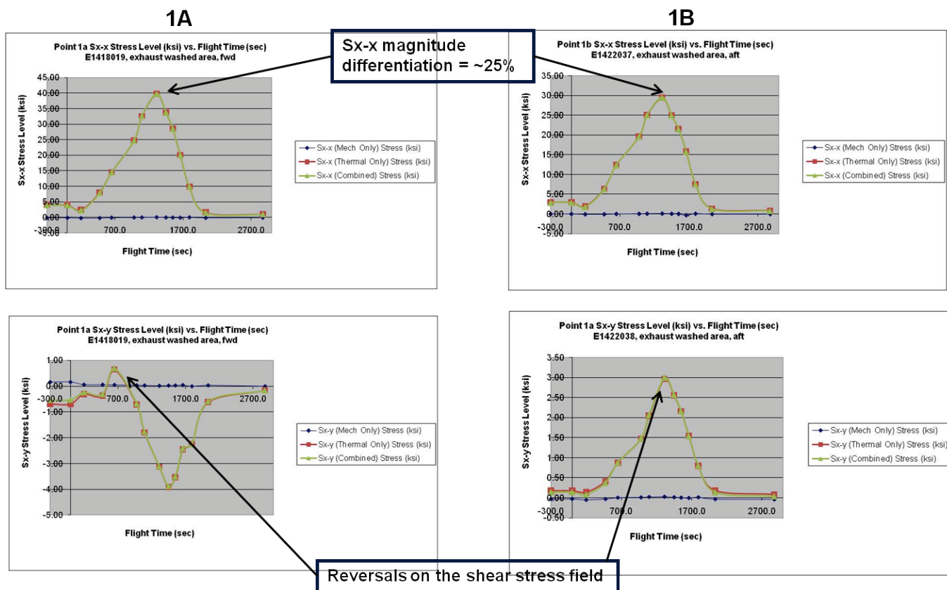
Figure 2.3.3 Panel 1A and 1B Stress Level vs. Flight Time Screening
