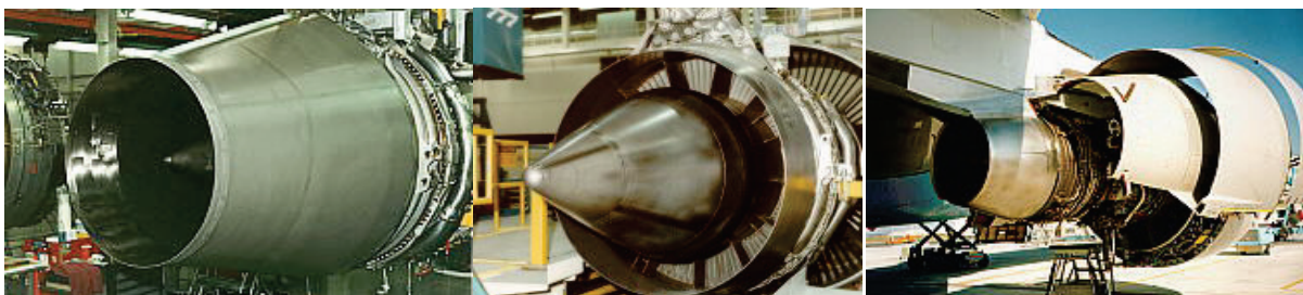
Figure 5.4.4 Examples of Uses of Titanium Honeycomb Sandwich Structures in Engine Nacelle Areas. Goodrich has also been instrumental in the design, development and use of nickel honeycomb sandwich structure dating back to the early 1970's. Design applications have since included the programs as the X-33, and many high temperature engine ducts.
