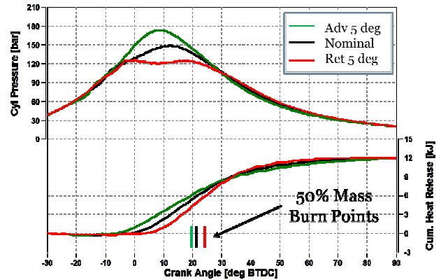
Figure 7: MFB50 vs. Combustion Phasing
