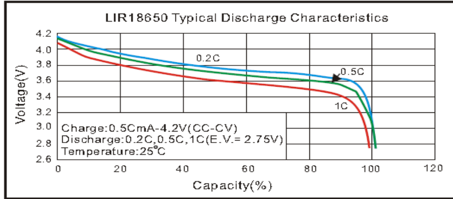
Figure 3: 18650 Discharge Characteristics
