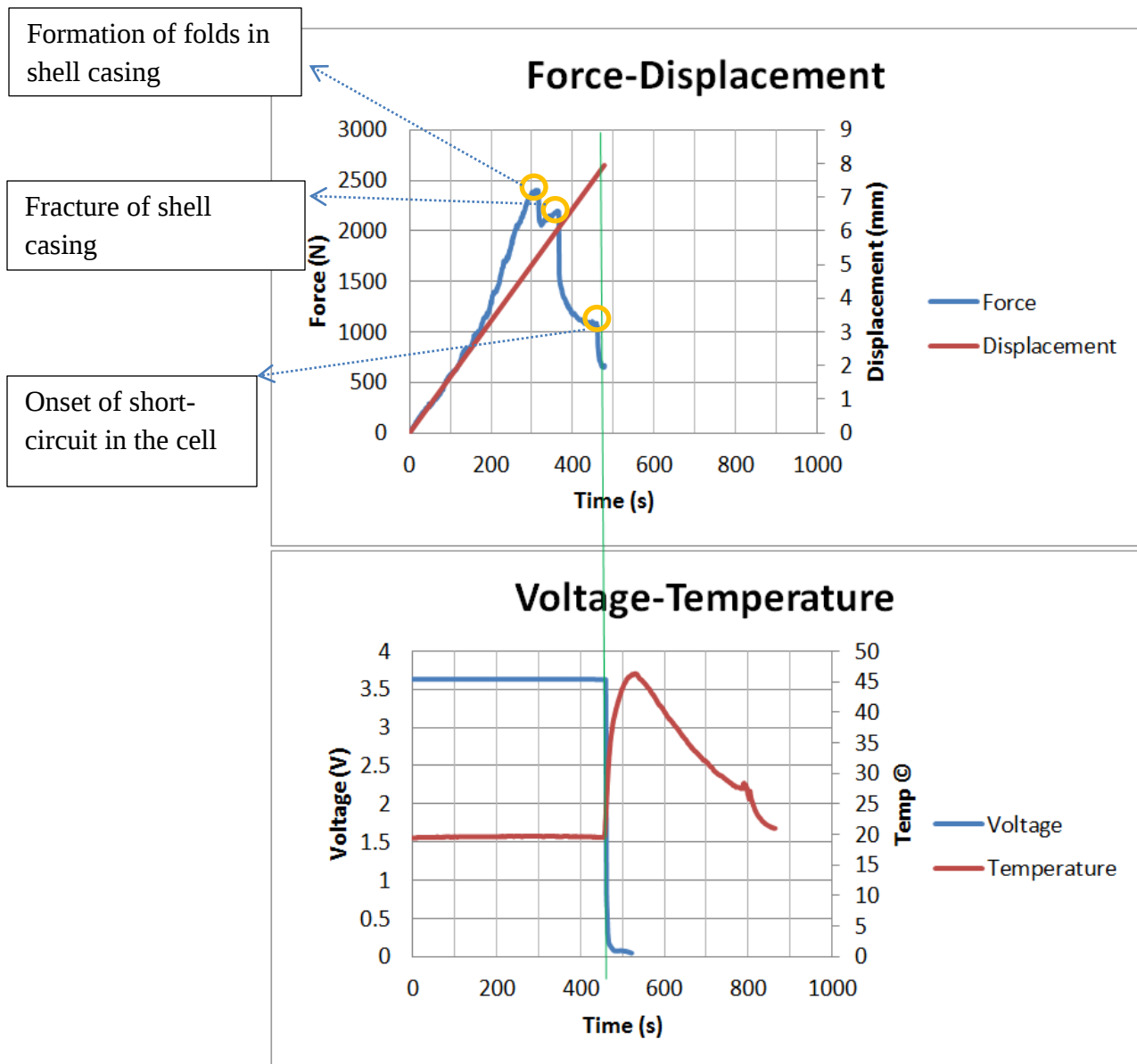
Figure 17: Force, displacement, voltage, and temperature measurements during three-point bending test
