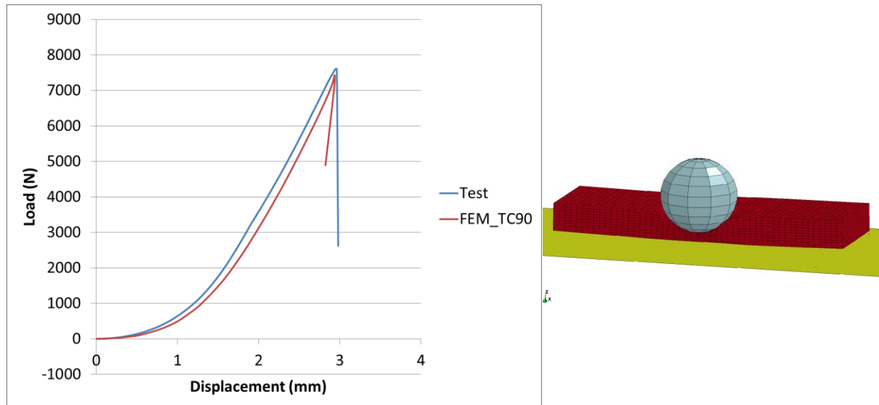
Figure 32 Comparison of Load Displacement curve between the updated FEM simulation and Test no.3 (left), Cross section of cell model at point of maximum deformation (right)
