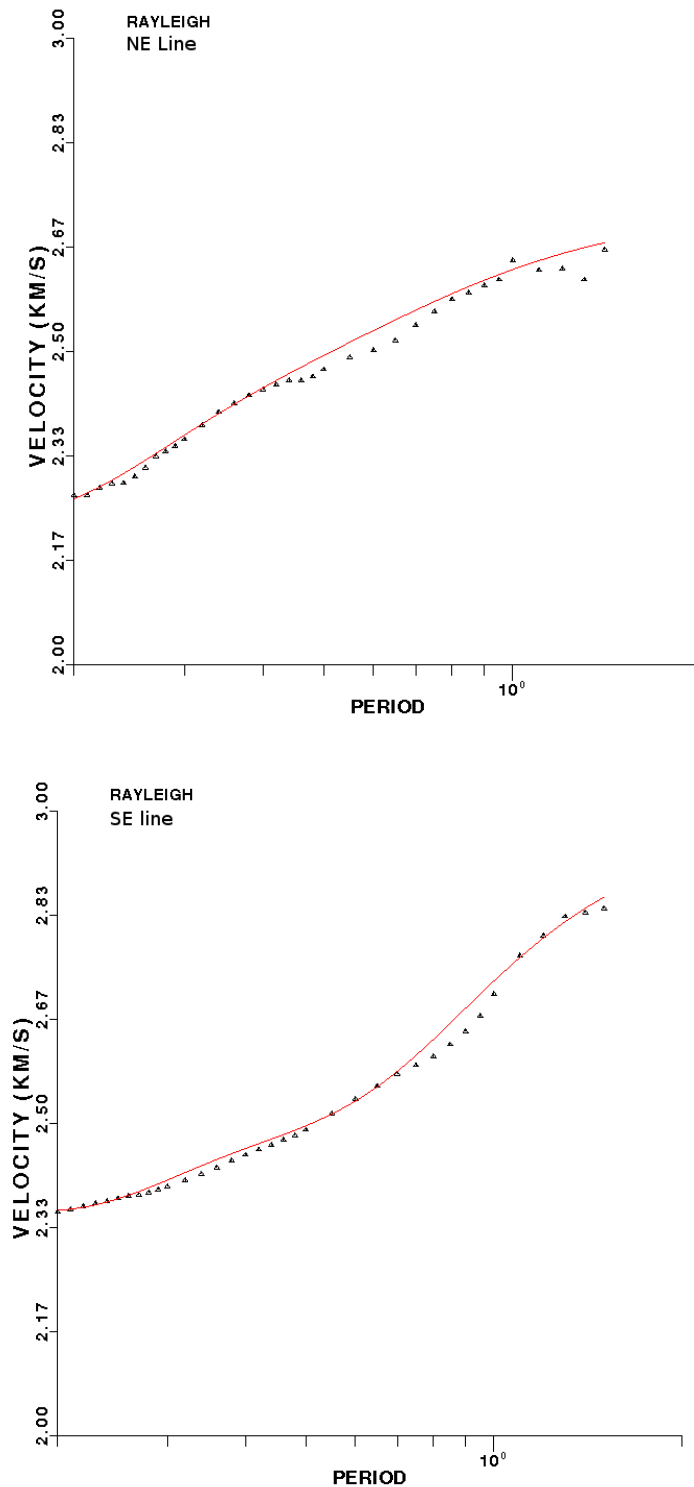
Figure 6. Average Dispersion Curves and Calculated Dispersion Curves from the Velocity Models
