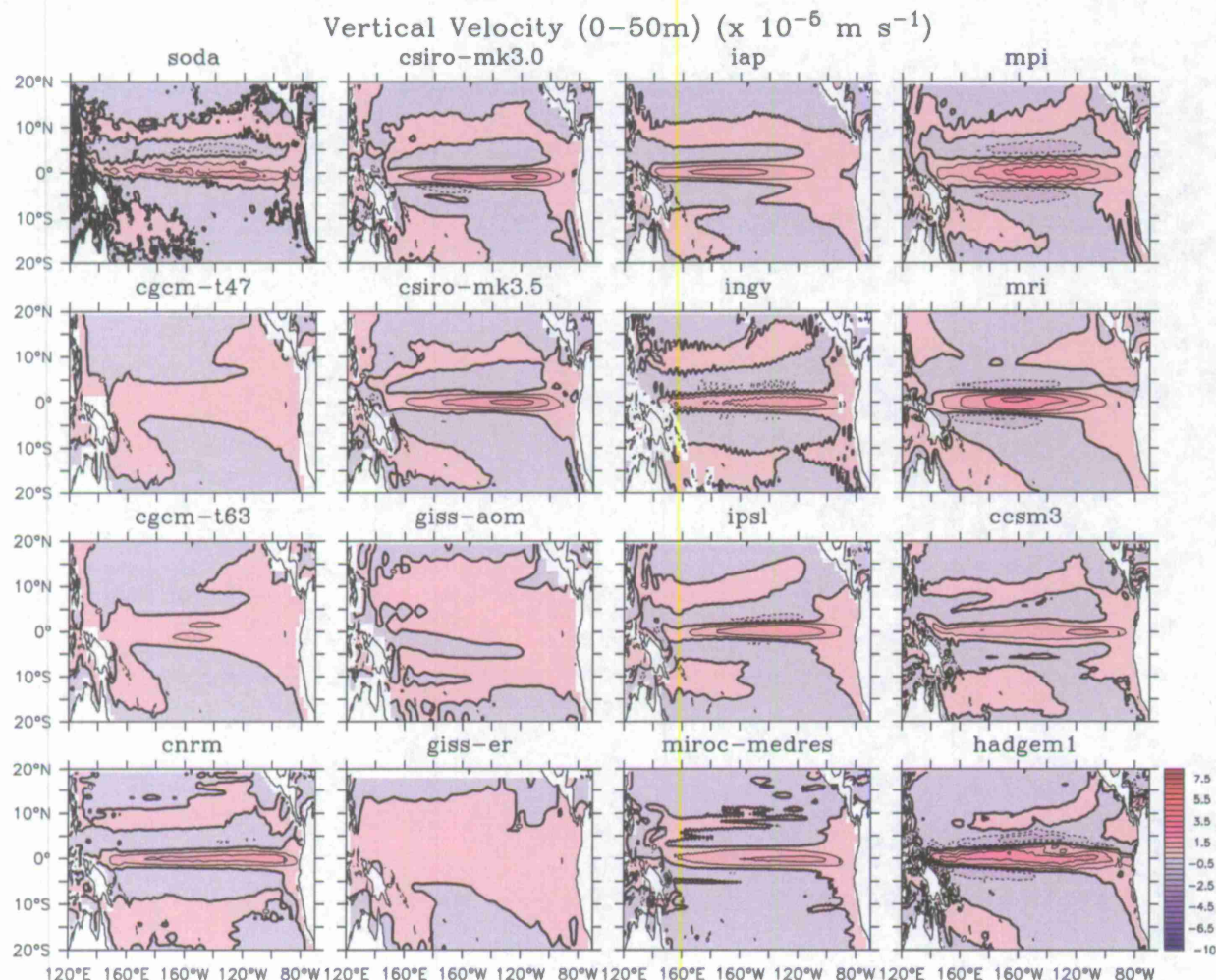
Figure 10. As in Figure 5, but for vertical velocity.
