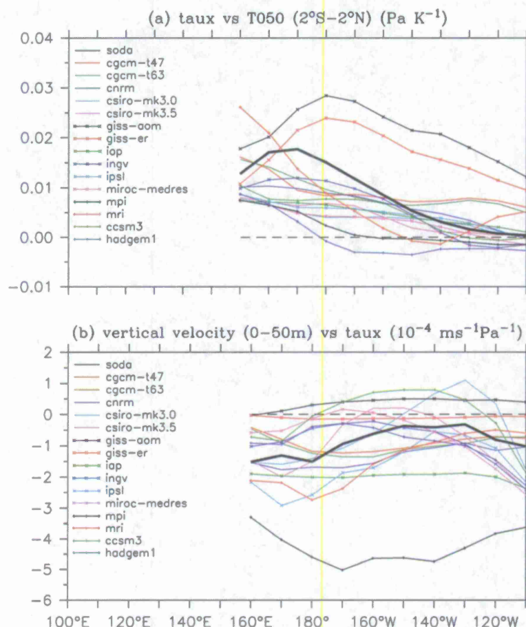
Figure 15. Linear regression of 2°S–2°N averaged of 20-year monthly mean data for (a) \tau_x vs T050 ( \text{Pa K}^{-1} ) and (b) vertical velocity (0–50 m) vs \tau_x ( \times 10^{-4} \text{ ms}^{-1} \text{ Pa}^{-1} ) from SODA ocean analysis and 15 IPCC AR4 CGCMs. The data are first converted to 10-degree bins in longitude before meridional averaging. The period for analysis is January 1980–December 1999.
