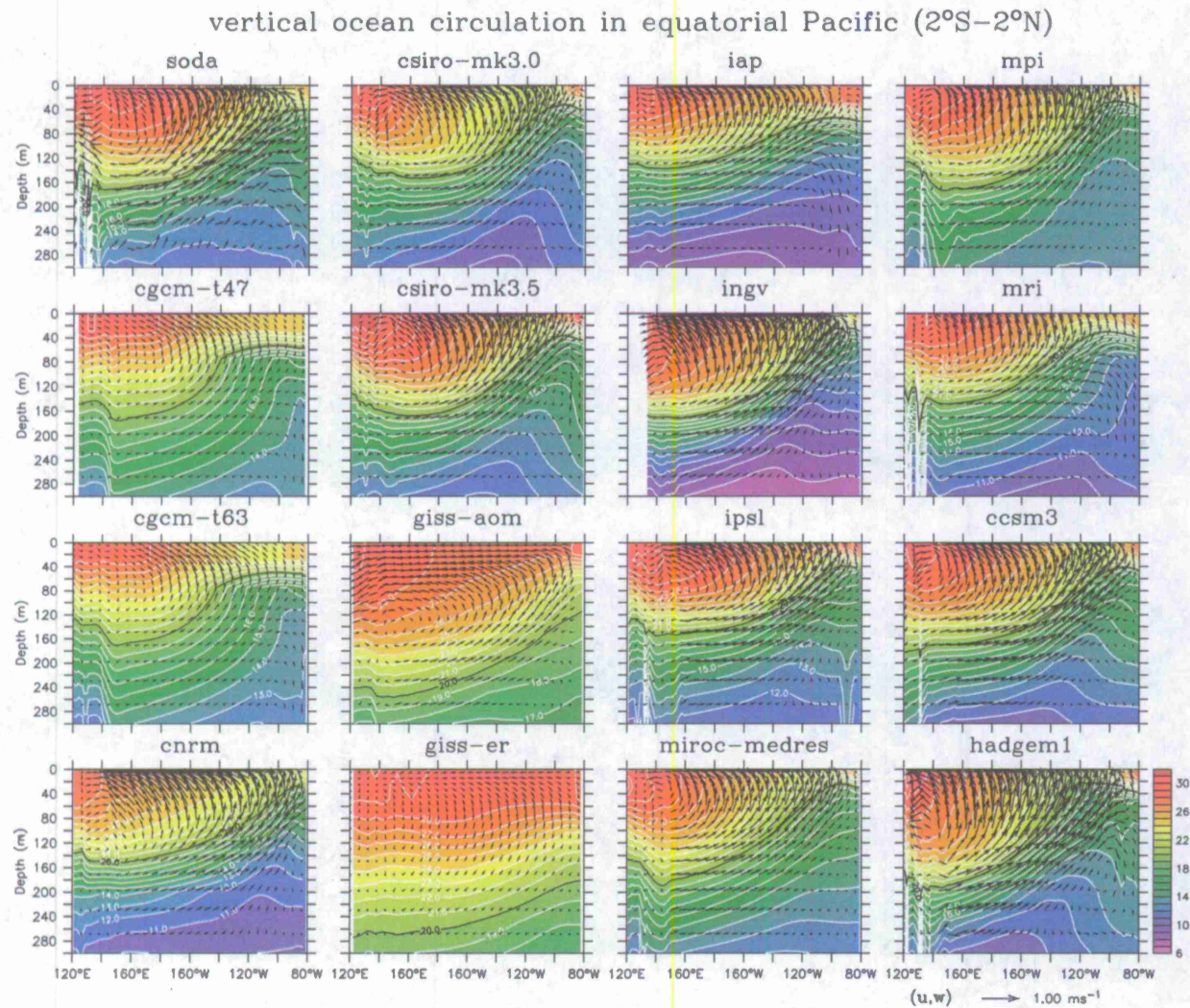
Figure 3. Annual mean vertical ocean circulation (vectors in \text{m s}^{-1} ) and temperature (shading contours in ^{\circ}\text{C} ) in the zonal-vertical plane averaged along 2^{\circ}\text{S} – 2^{\circ}\text{N} from monthly data in SODA ocean analysis and 15 IPCC AR4 CGCMs. 20^{\circ}\text{C} isotherm is denoted by the black curve. The period for averaging is January 1980–December 1999.
