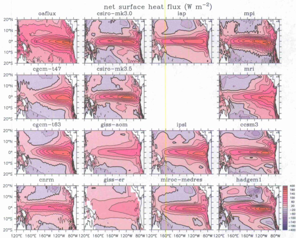
Figure 4. Temporal mean net surface heat flux ( \text{W m}^{-2} ) in the tropical Pacific Ocean from OAFlux and 14 IPCC AR4 CGCMs. The period for averaging is July 1983–December 1999.
