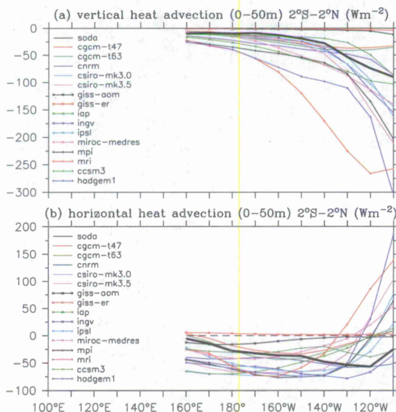
Figure 9. Annual mean (a) vertical and (b) horizontal heat advection ( \text{W m}^{-2} ) in the upper 50 m averaged along 2°S–2°N from monthly data in SODA ocean analysis and 15 IPCC AR4 CGCMs. The data are first converted to 10-degree bins in longitude before meridional averaging. The period for averaging is January 1980–December 1999.
