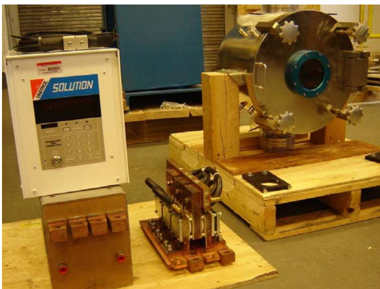
Figure 1. Controller, power supply, and environmental chamber for electromechanical joining system.
