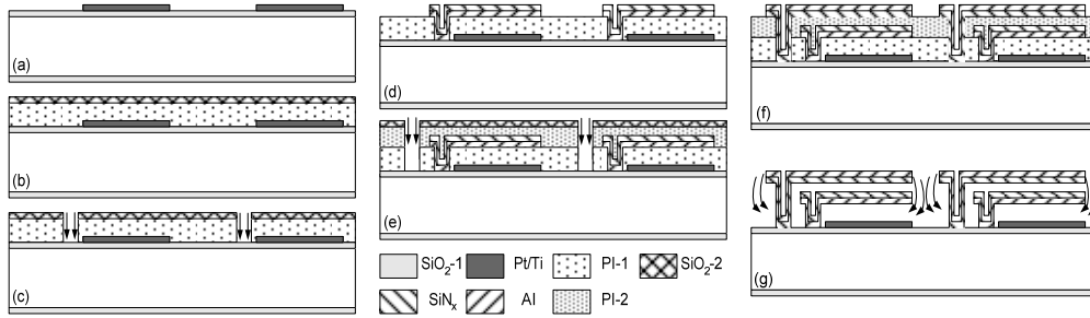
Fig. V-3: Fabrication process of the double-cantilever microbolometer FPAs: (a) 150 nm-thick Pt/Ti wires and pads by standard lift-off process on thermal-oxidized silicon wafers, (b) spin-on coating and curing of 2.5 \mu\text{m} -thick polyimide and deposition of a 500 nm-thick etching mask layer of PECVD SiO 2 , (c) etching of SiO 2 by RIE with SF 6 and He and anisotropic etching of polyimide by RIE with O 2 , (d) the bottom bimaterial cantilever of a 200 nm-thick PECVD SiN x layer and a 200 nm-thick Ebeam Al layer, (e) the second sacrificial layer of 1- \mu\text{m} thick polyimide, (f) the top bimaterial cantilever of a 200 nm-thick Ebeam Al layer and a 200 nm-thick PECVD SiN x layer, and (g) release of the microbolometer FPAs by isotropic etching of both polyimide layers with O 2 plasma.
