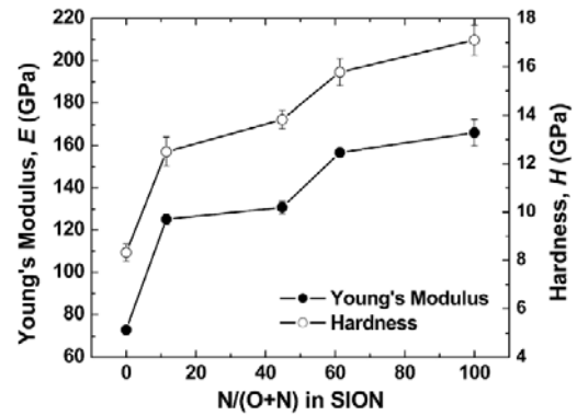
Fig. VI-6: Young's modulus and indentation-hardness of the SiON films as a function of the nitrogen content [N/(O + N)] .
