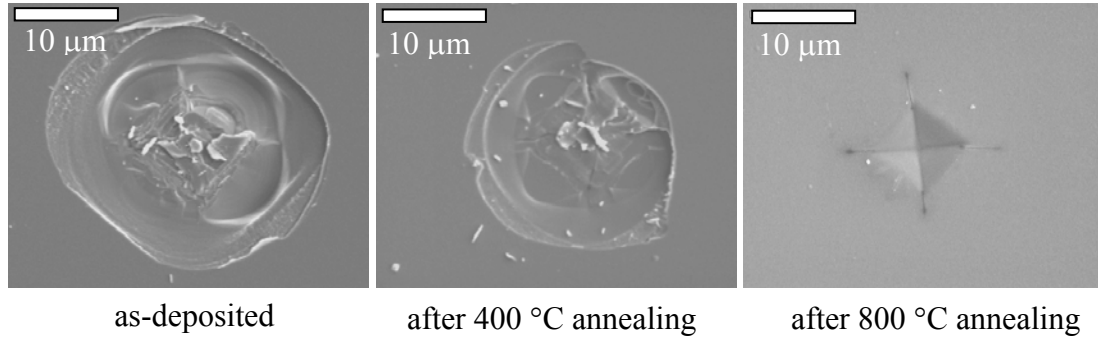
Fig. IX-4: SEM images of delamination on the \text{SiO}_x films after indentation.
