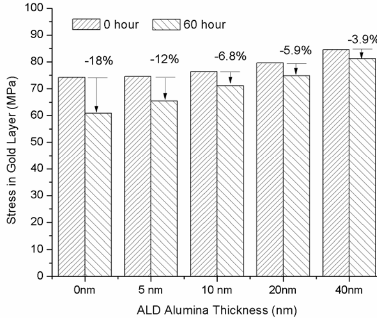
Fig. X-12: The relationship between ALD alumina thicknesses and tensile stress relief in Au layer after 150 °C isothermal holding.
