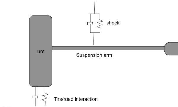
Figure 16. Simple dynamic model of suspension
