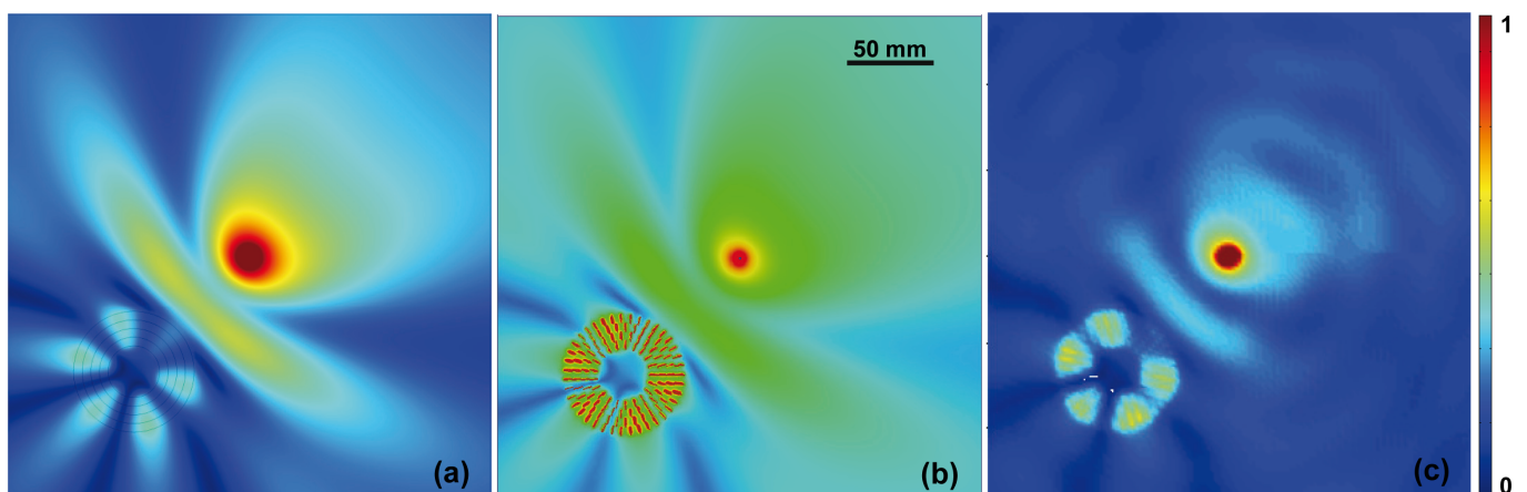
Figure 5 | E-field complex magnitude map for a point source illuminating the RPC shell (source – center separation r = 95 mm) and radiating at f = 3.8 GHz ( q = 3 mode): (a) analytical simulation; (b) ab-initio simulation; (c) measurement results. Field scale is normalized with respect to the maximum value in each plot.
