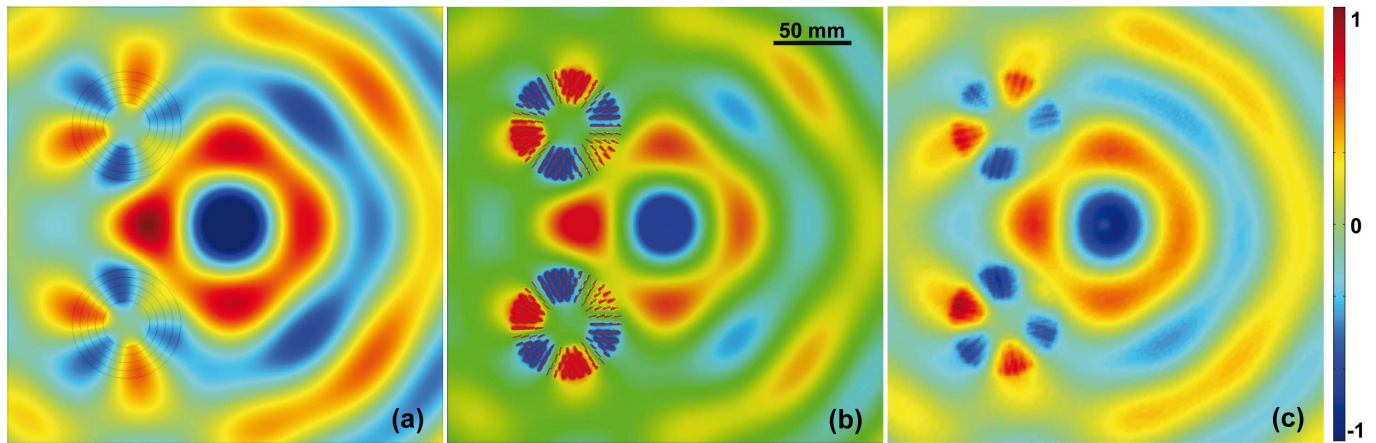
Figure 6 | Real part of the E-field for a point source illuminating 2 RPC shells at a distance of approximately 90 mm to their centres and radiating at a frequency f = 3.8 GHz ( q = 3 mode): (a) analytical simulation; (b) ab-initio simulation; (c) measurement results. Field scale is normalized with respect to the extreme values in each plot.
