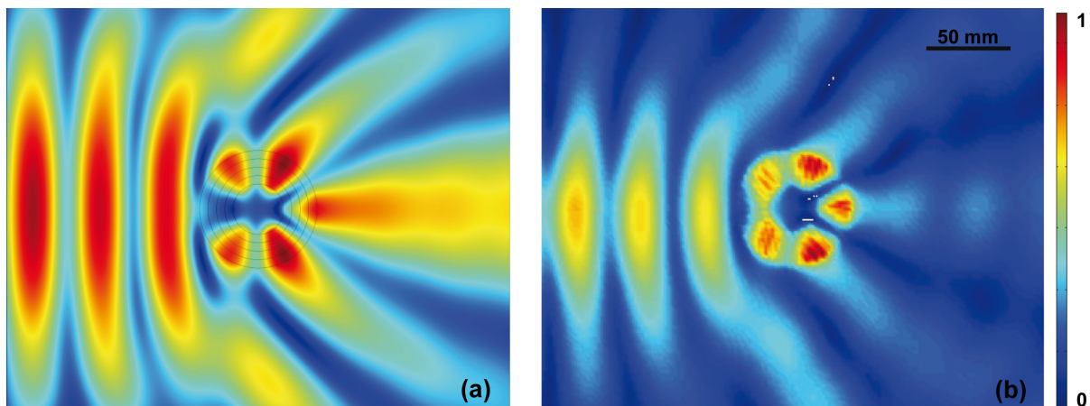
Figure 7 | E-field complex magnitude map for a plane wave illuminating an RPC shell at a frequency f = 3.8 GHz ( q = 3 mode): (a) analytical simulation; (b) measured results. Results in (a) include a deformed (slightly bended) wave shape according to the practical setup characteristics. Field scale is normalized with respect to the maximum value in each plot.
