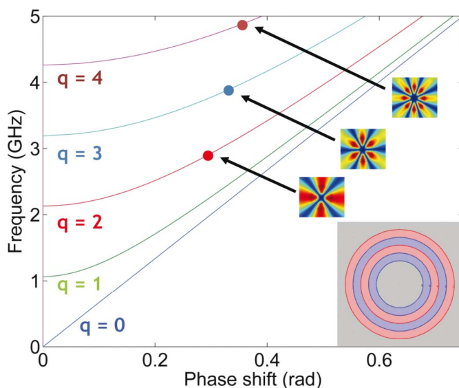
Figure 1 | Dispersion diagram of the ideal RPC structure with full set of constitutive parameters. Cut-off frequencies of modes with q > 0 are equally spaced (aprox. 1.1 GHz). Lower right inset represents a 4 layers (finite size) device with internal cavity of radius r = 15 mm and periodicity d_a = d_b = 5 mm. Dots and associated E-field patterns correspond to the resonance frequencies of the selected operation mode ( q = 3 ; f = 3.8 GHz) and adjacent ones of the 4-layers RPC shell.
