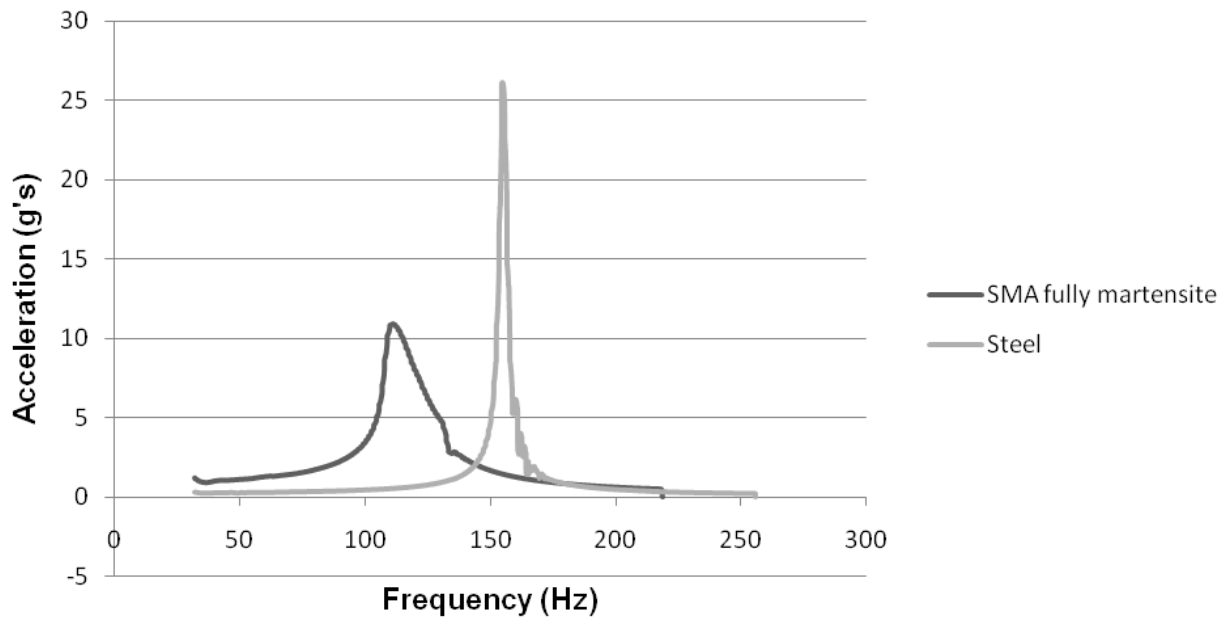
Figure 24 – Comparison of martensitic SMA with steel in sine upsweep
