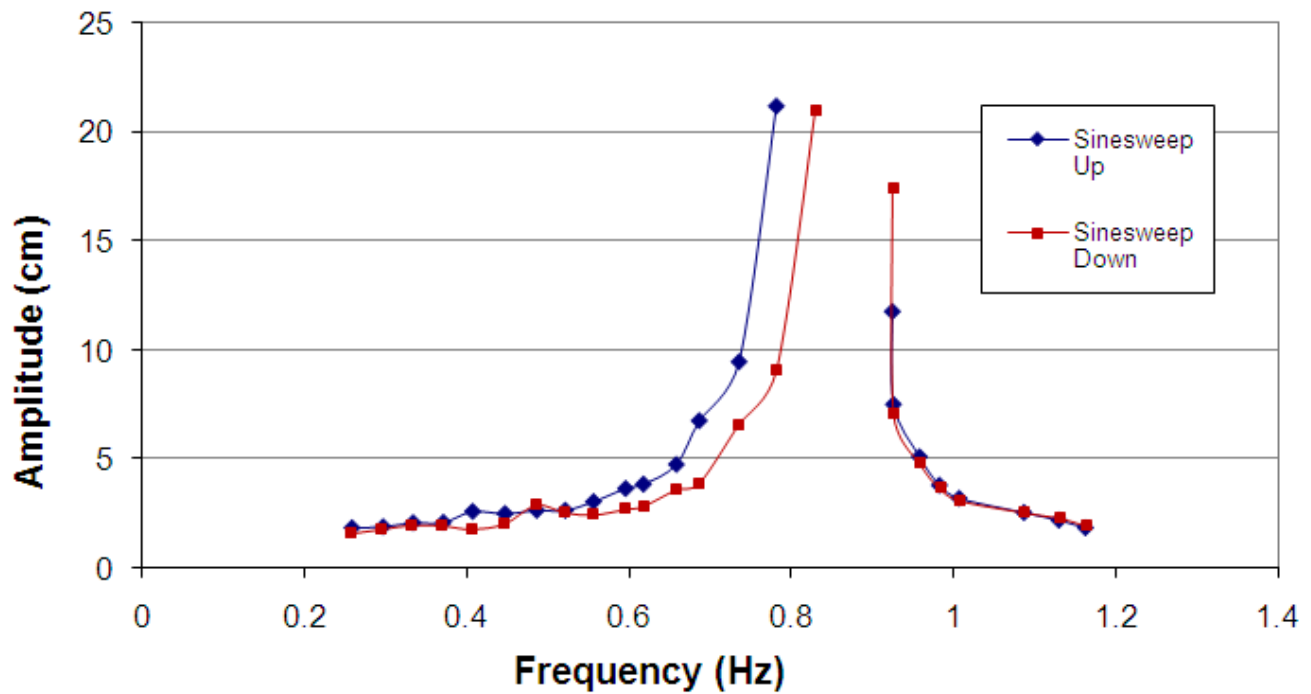
Figure 7 - Frequency response of steel spring system
