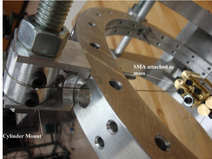
Figure 19 – Cylinder mounts for SMA wires
