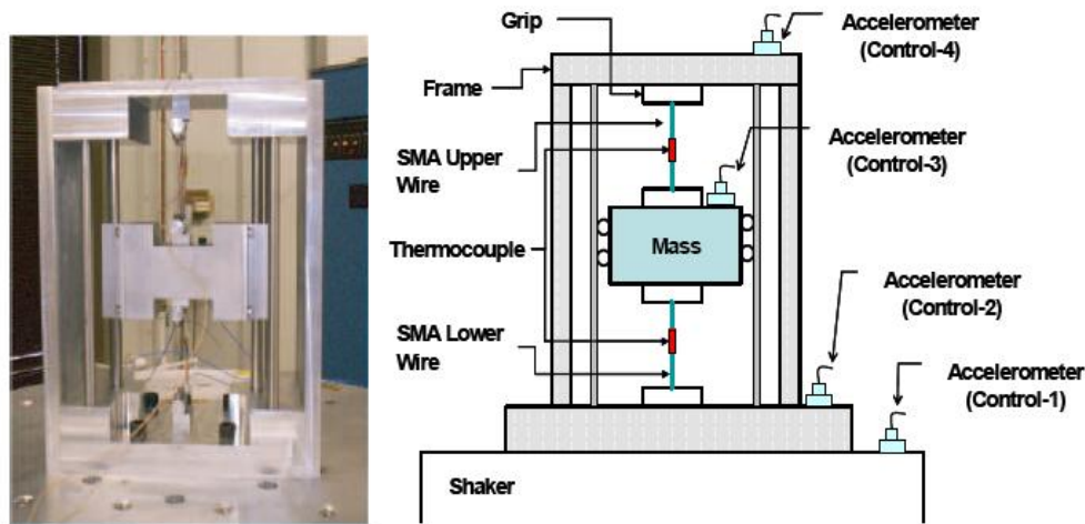
Figure 14– Setup for one degree of freedom vibration experiment
