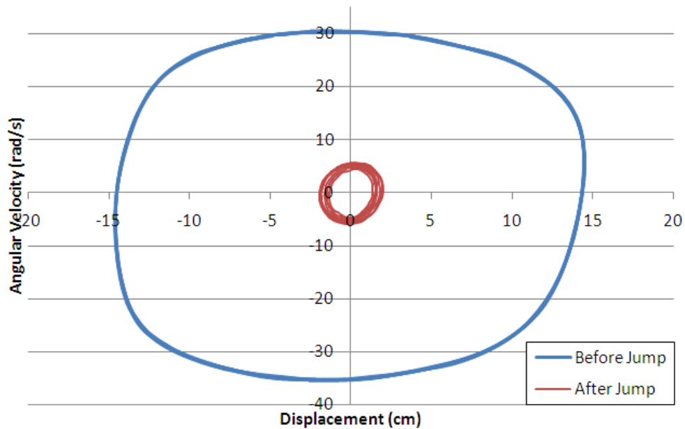
Figure 10 - Angular velocity vs. displacement for SMA springs
