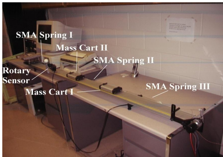
Figure 11 – Two degree of freedom mass cart system
