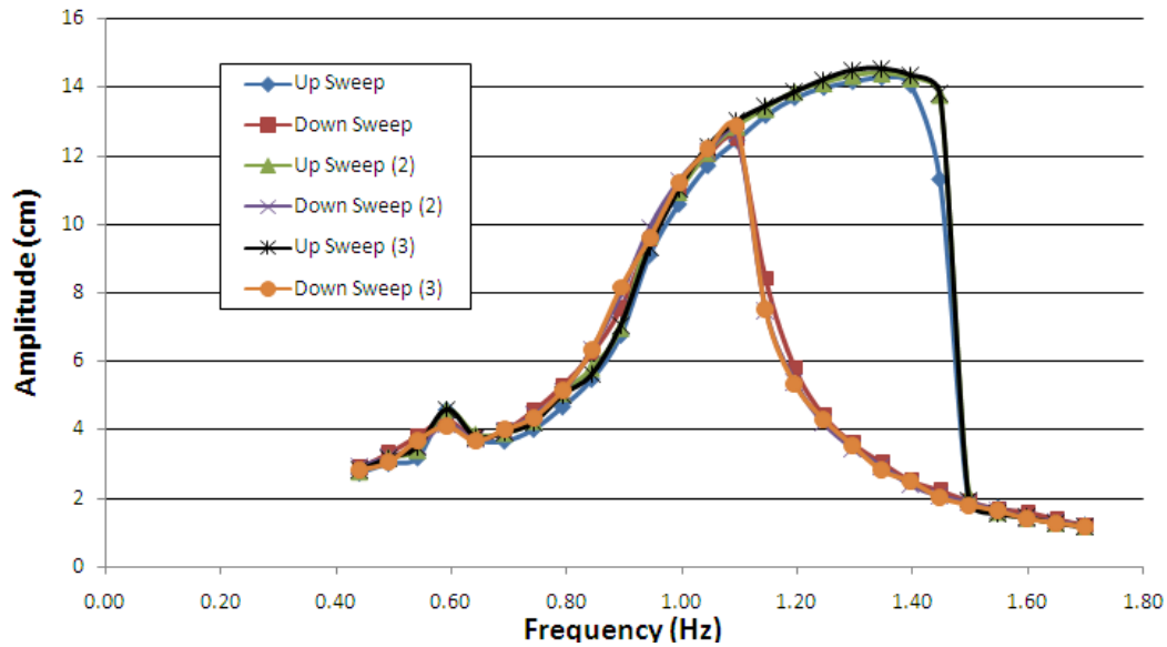
Figure 9 - Frequency response for SMA springs
