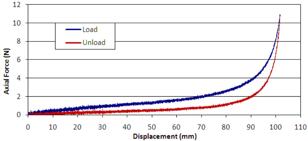
Figure 5 - Force vs. displacement for SMA spring
