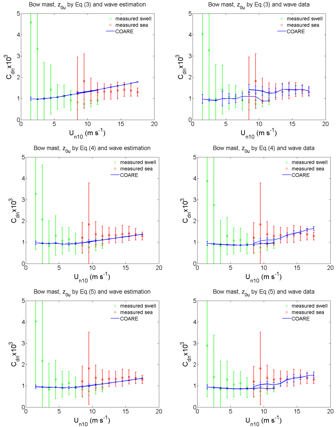
Figure 5. Neutral drag coefficient C_{dn} against neutral wind speed at 10 m above sea level U_{n10} in wind bins of 1 \text{ m s}^{-1} with standard deviation and with z_{0u} estimated from Eqs. (3), (4) and (5).
