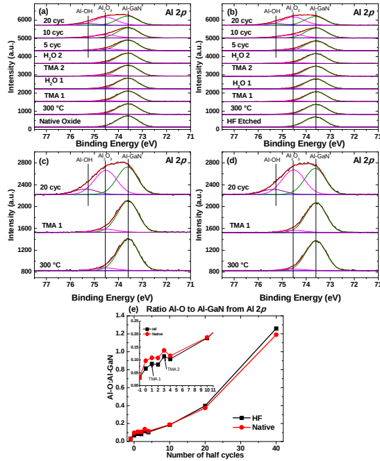
Figure 5. Al 2 p core level spectra from the native oxide (a, c) and HF etched (b, d) samples at various stages in the Al 2 O 3 deposition process. (e) The ratio of Al-O to Al-GaN from the same spectra indicating the change in Al 2 O 3 growth rate with increasing number of ALD cycles. Inset shows the change in ratio during the initial ALD cycles.
