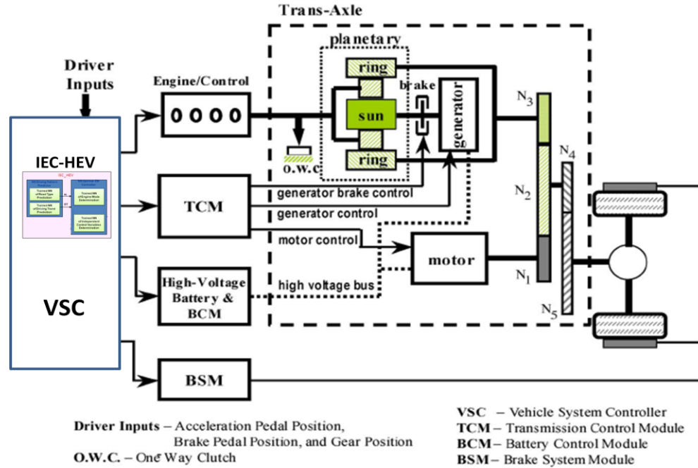
Figure 1. Power Split HEV configuration into VSC
