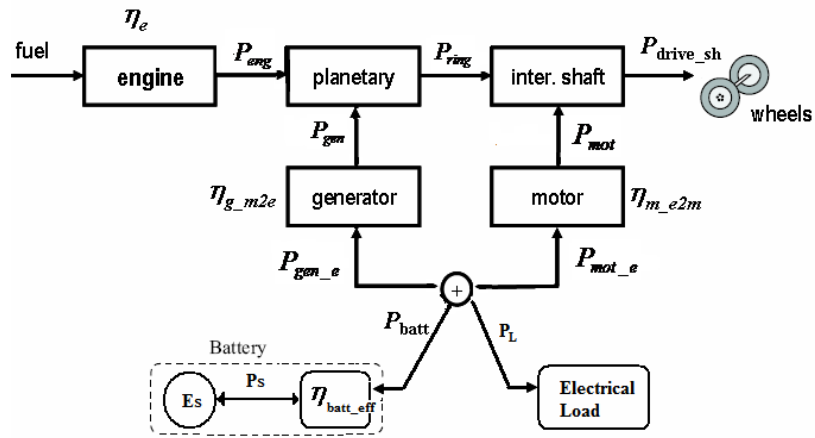
Figure 2. Power flow in a Split HEV configuration with arrows indicating positive power.
