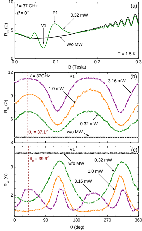
Figure 5.6 This figure examines the angular response of R_{xx} at different microwave power levels, P . (a) Magnetoconductance oscillations in R_{xx} are exhibited for f = 37 GHz with \theta = 0 and P = 0.32 mW. (b) shows the \theta dependence of R_{xx} of the principal maximum P1. (c) shows the \theta dependence of R_{xx} of the principal minimum V1. In these figures, the w/o MW (w/ MW) traces indicate the sample response in the absence (presence) of microwave photo-excitation. Note that, in (c), additional peaks occur near \theta = 45^\circ and \theta = 225^\circ at P = 3.16 mW.
