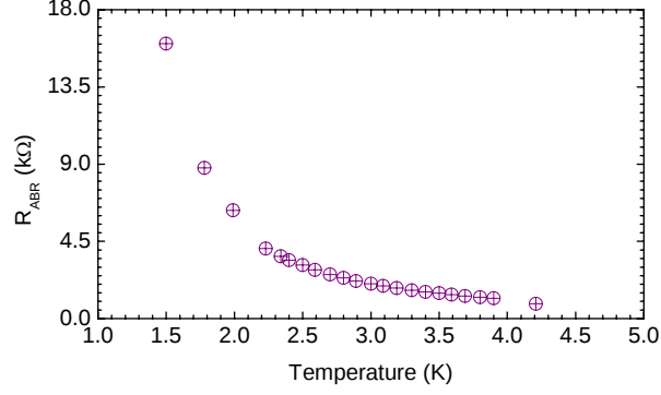
Figure A.5 ABR resistance vs temperature is shown for 75 \Omega ABR. Current through the resistor is 0.5 \mu A.
