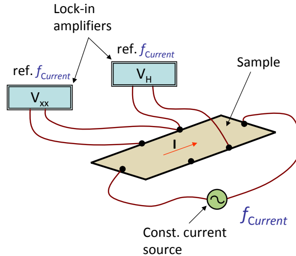
Figure B.1 Schematic of the electrical connections for a typical measurement is shown. A constant current source sends a low frequency, f_{current} , AC current through the specimen, and the same frequency is used as the reference of the lock-in amplifiers, which measure the voltages across given two contacts.
