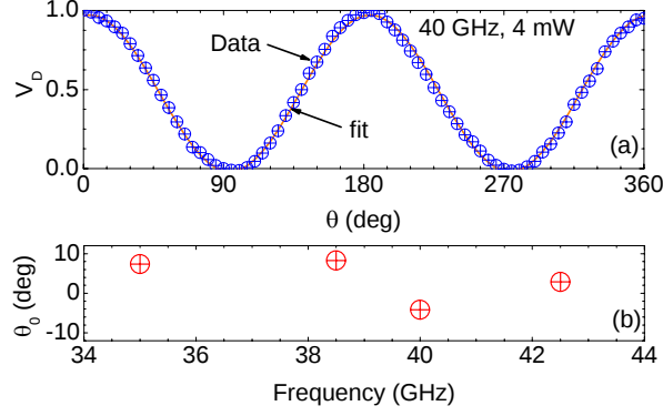
Figure 5.2 (a) Normalized detector response vs the polarization angle is shown for 40 GHz. (b) The phase shift obtained from NLSFs for different frequencies.
