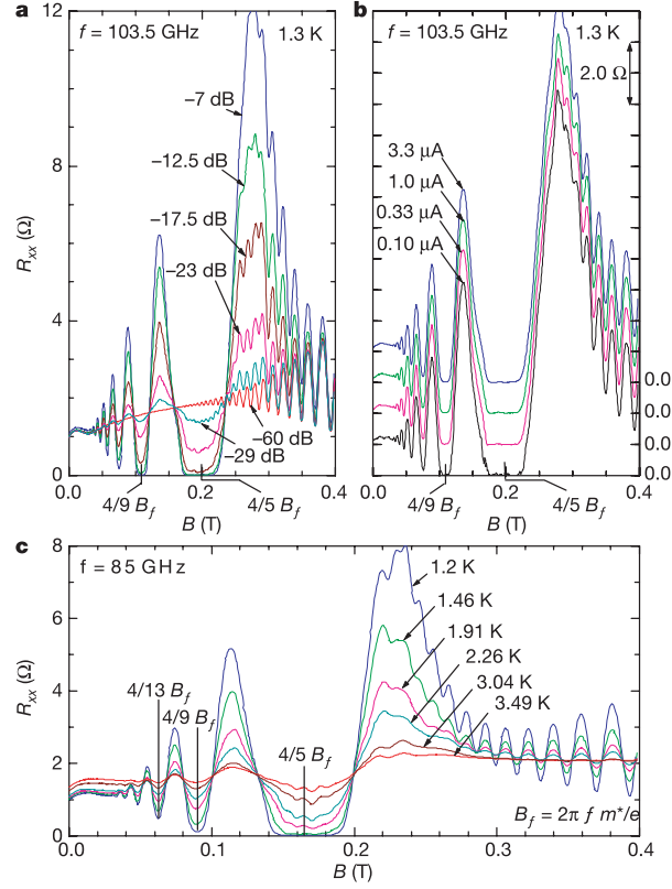
Figure 3.4 (a) Microwave power, (b) DC current, and (c) temperature dependence of MIMO. After Mani et al. (2002). [11]
