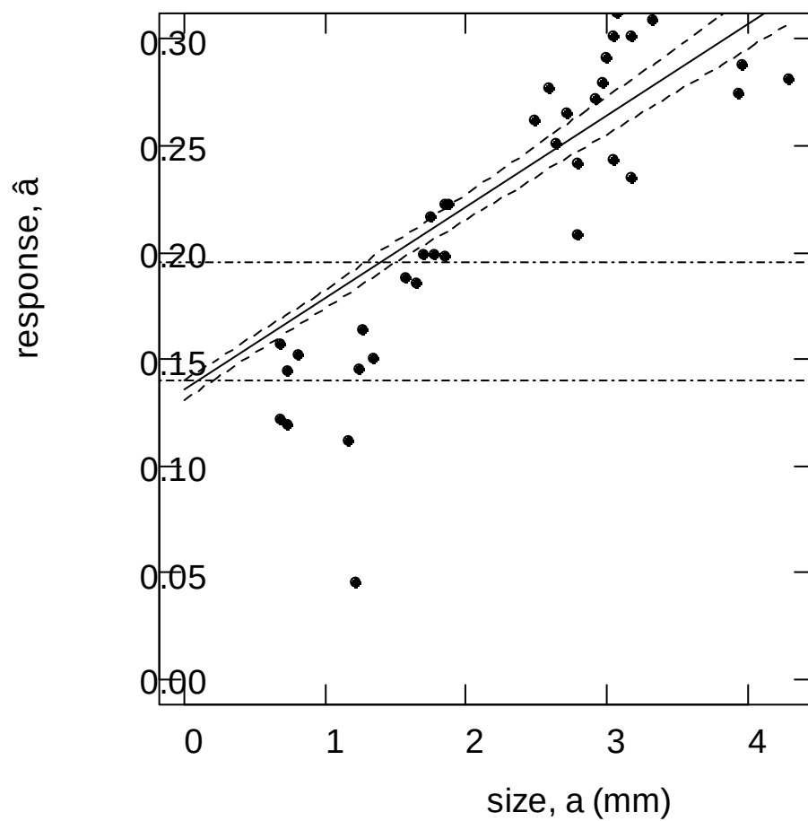
Figure 6. Linear model fit for data with square-root transformation.
