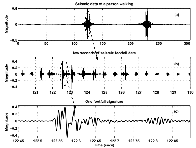
Figure 8. (a) Seismic data of a person walking, (b) enlarged portion – shows the periodicity of footsteps and (c) signature of one footprint
