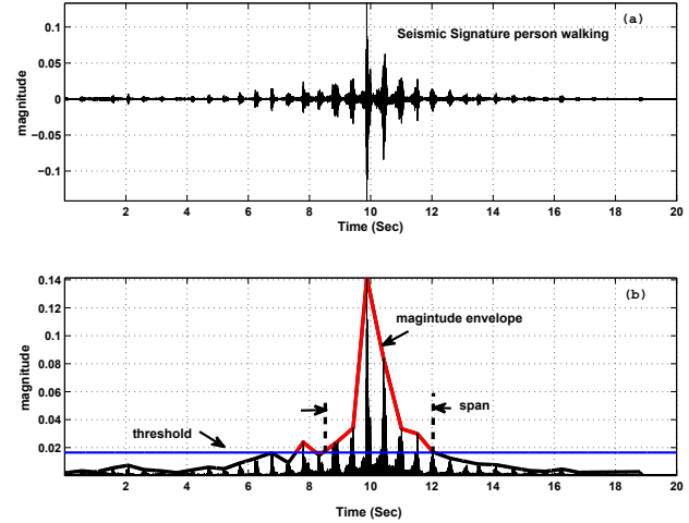
Figure 11. (a) Seismic signals generated by a person walking, and (b) signal span for a person walking
