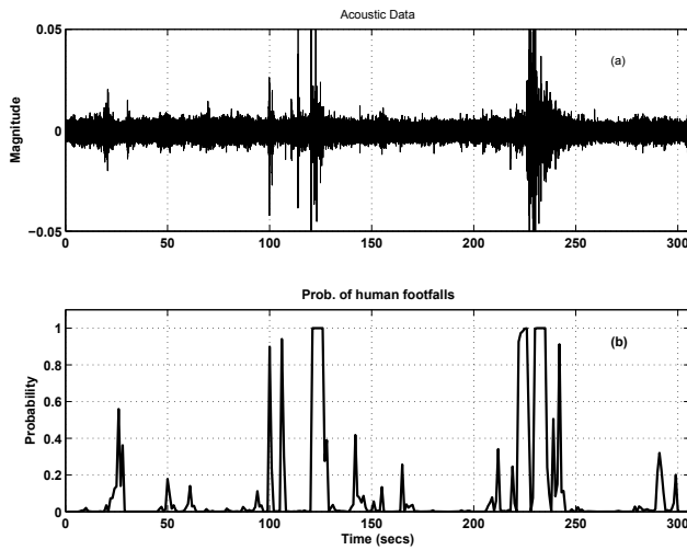
Figure 7. (a) Acoustic data of a person walking and (b) Probability of acoustic footprint detection
