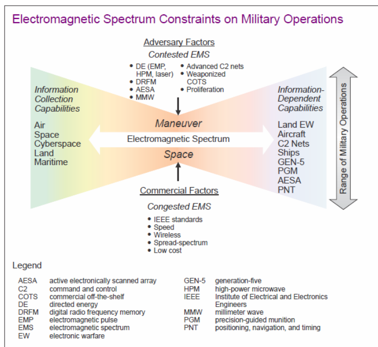
Figure I-1. Electromagnetic Spectrum Constraints on Military Operations
