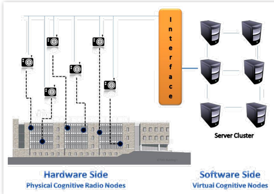
Figure 6.2: Indoor Cognitive Radio Network Testbed (CORNET) used at Virginia Tech for Radio Resource Management Research. The test bed consists of 48 agile radio nodes to test dynamic spectrum access, spectrum security, location dependent radio management and policy (radio environment maps), and other technologies.
