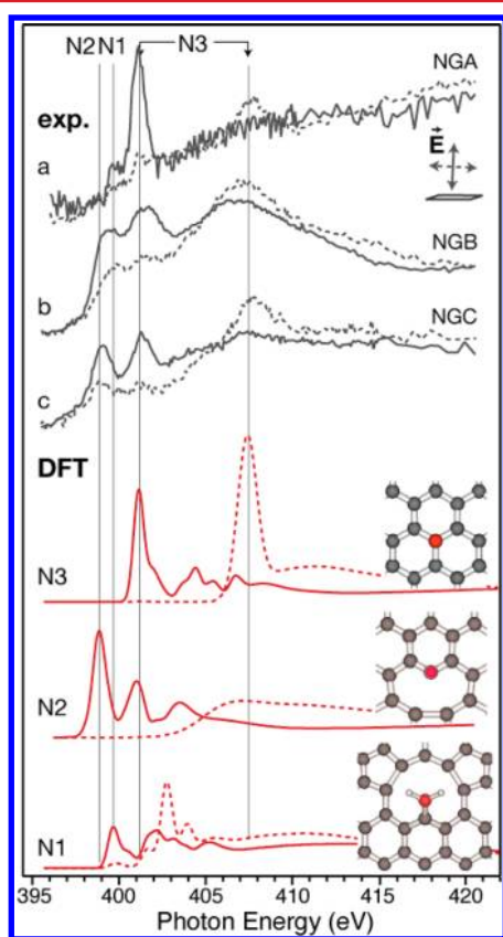
Figure 3. Experimental N 1s XAS (gray curves) measured in PEY mode for (a) NGA (on Cu); (b) NGB transferred to SiO 2 ; (c) NGC (on Cu) exposed to ambient atmosphere, and DFT-computed spectra (red curves) for cluster models of graphitic (N3); pyridinic (N2); and nitrile-like (N1(+H)) nitrogen dopants, used to assign the experimental resonances. Solid and dashed lines indicate out-of-plane and in-plane intensity, respectively, in the computed spectra; the measurements were taken at grazing incidence of 20° (solid line) and 70° (dashed line).
