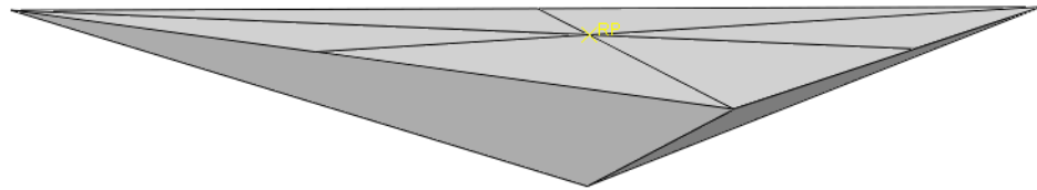
Figure II.1-12: 3D model of Berkovich indenter.
