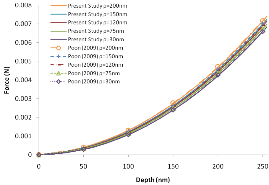
Figure II.1-6: Load–displacement comparison for elastic indentation simulation into a specimen with varying indenter tip radii, \rho (30, 75, 120, 150 and 200 nm).
