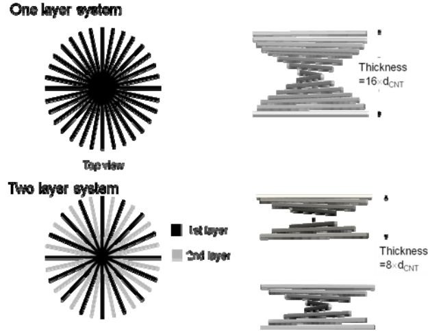
Figure 3. The fan-out pattern of our volume cell is horizontally along the radial direction at every 22° each, the closed packaging of N p =16 NIR CNTs must be overlaid passing one another in the central core creating a stack of tubes like a fireman spiral staircase.
