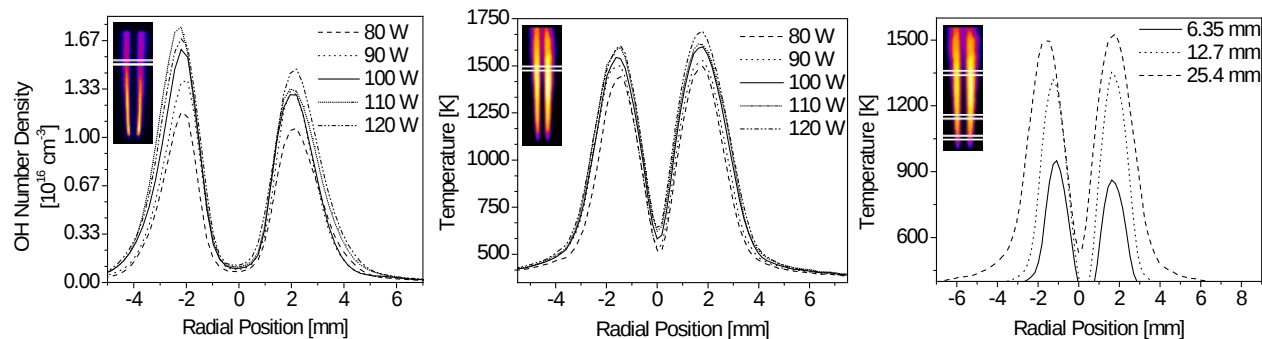
Figure 26. OH number density (left) and temperature (center) profiles of the premixed hollow electrode plasma discharge for varying power levels with inset images depicting area of data extraction (25 mm over torch). Temperature profile at three downstream locations in a flame with an equivalence ratio of 6.0
