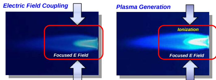
Figure 9. Schematic of direct plasma coupling (low microwave power (left), high microwave power (right)). stabilization mechanism [40].
