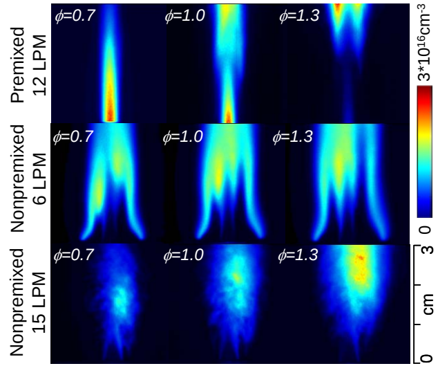
Figure 8. Averaged OH PLF images for all flowrates at premixed mode with \phi = 0.7, 1.0 and 1.3 (top); Averaged OH PLF images for 6 LPM (middle)/15 LPM (bottom) at non-premixed mode with \phi = 0.7, 1.0 and 1.3 .
