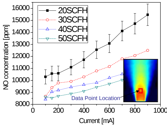
Figure 5. Nitric oxide concentrations in the reaction zone of the flame for plasma only case with air (left), and plasma with combustion (right). Methane and air flame is used at \phi=1 for various flowrates.
