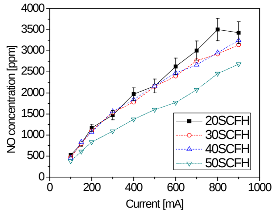
Figure 5. Nitric oxide concentrations in the reaction zone of the flame for plasma only case with air (left), and plasma with combustion (right). Methane and air flame is used at \phi=1 for various flowrates.
