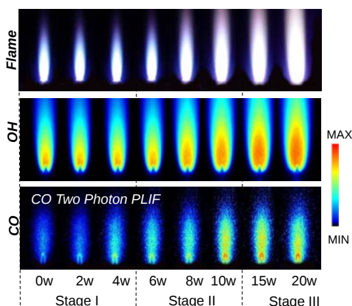
Figure 12. Photo (top), OH PLIF (middle) and CO PLIF (bottom) intensity images of CH 4 /O 2 flame vs. microwave power with three stages noted (100 SCCM total flowrate at \phi=1.1 )
