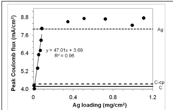
Figure 16. Oxygen reduction activity of carbon-conductive polymer-silver (C-cp-Ag) as a function of Ag loading under oxygen atmosphere. Planar silver (Ag), uncoated carbon (C), and carbon-conductive polymer (C-cp) are shown as reference.
