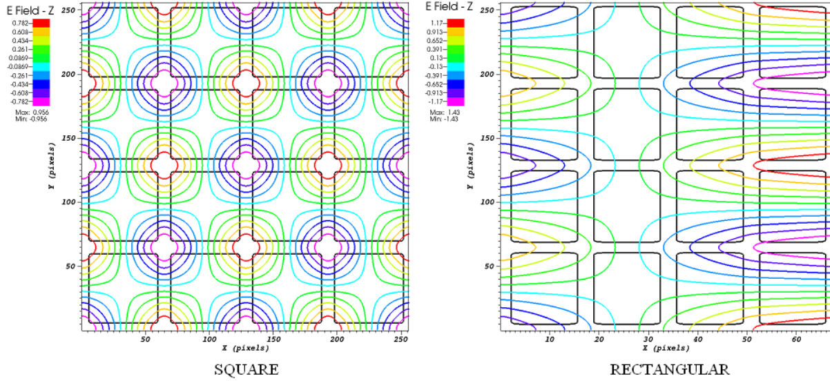
Figure 23. Real part of E_z for the fundamental TM mode computed at (left) k-point (wave vector) 2\pi/a (0.5,0.5,0) in the square lattice and at (right) k-point 2\pi/a (0.5,1.9,0) in the rectangular lattice. Vein dielectric permittivity 8.90
