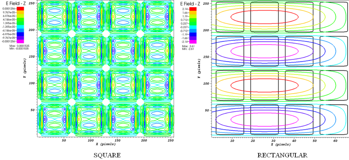
Figure 28. Real part of E_z for the TM mode at the second modal frequency computed at (left) k -point (wave vector) 2\pi/a (0.5,0.5,0) in the square lattice and at (right) k -point 2\pi/a (0.5,1.9,0) in the rectangular lattice. Vein dielectric permittivity 1.52
