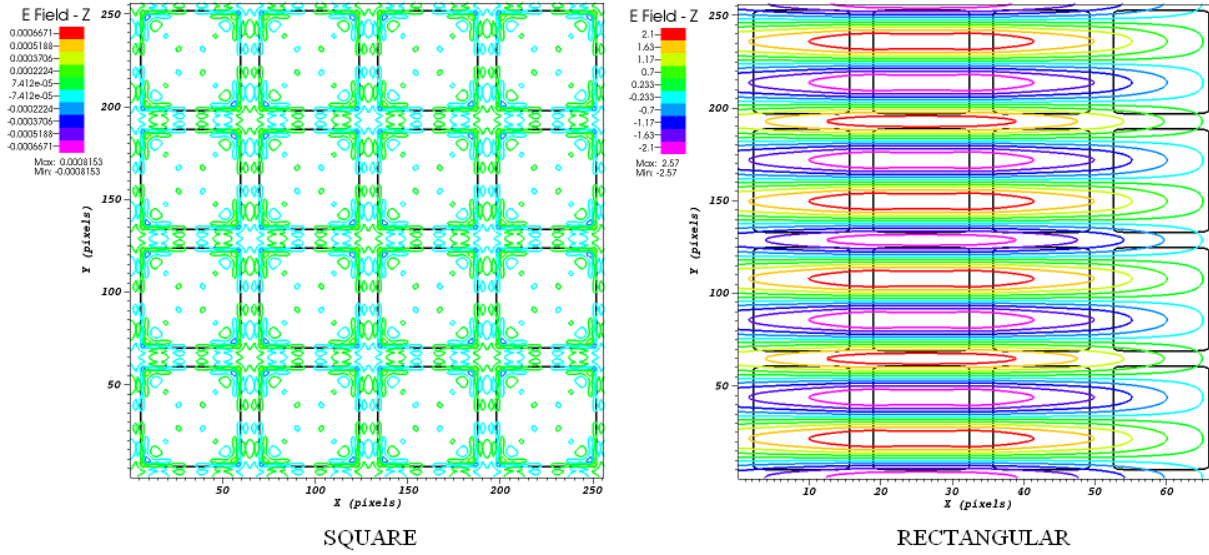
Figure 29. Real part of E_z for the TM mode at the third modal frequency computed at (left) k -point (wave vector) 2\pi/a (0.5,0.5,0) in the square lattice and at (right) k -point 2\pi/a (0.5,1.9,0) in the rectangular lattice. Vein dielectric permittivity 1.52
