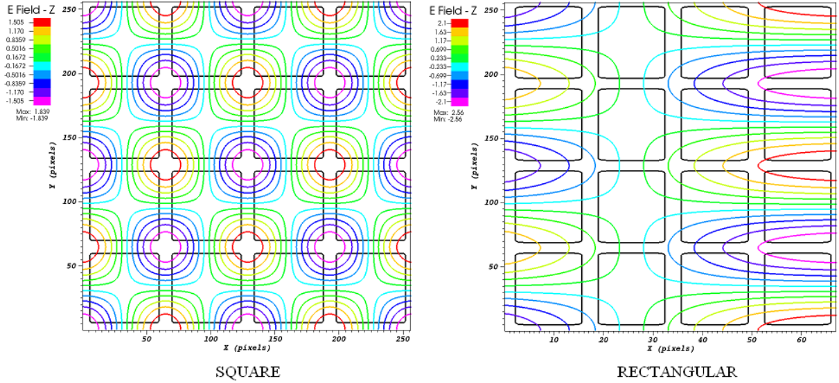
Figure 27. Real part of E_z for the fundamental TM mode computed at (left) k -point (wave vector) 2\pi/a (0.5,0.5,0) in the square lattice and at (right) k -point 2\pi/a (0.5,1.9,0) in the rectangular lattice. Vein dielectric permittivity 1.52
