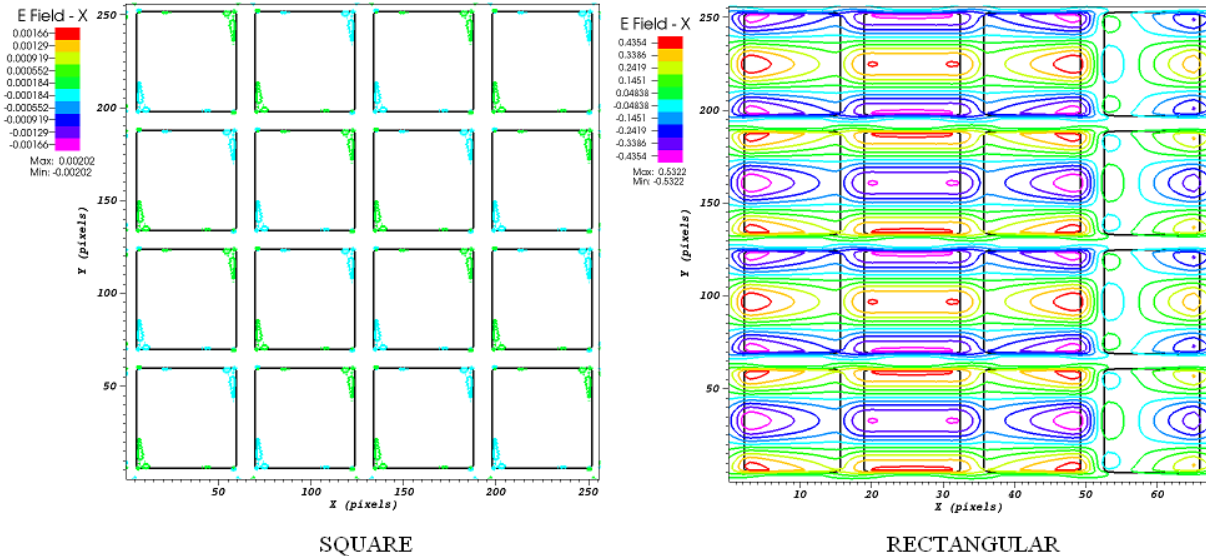
Figure 13. Real part of E_x for the third frequency computed at (left) k-point (wave vector) 2\pi/a (0.5, 0.5, 0) in the square lattice and at (right) k-point 2\pi/a (0.5, 1.9, 0) in the rectangular lattice. Vein dielectric permittivity 8.90
