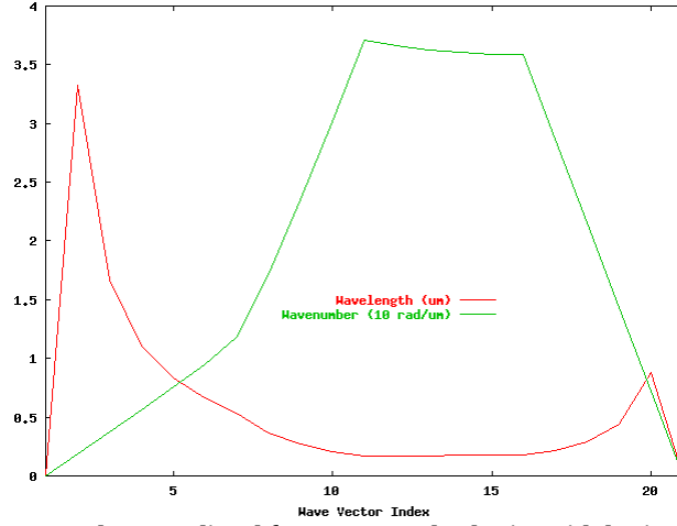
Figure 30. Wavelengths and wave numbers predicted for a rectangular lattice with lattice constant set at 0.333 \mu\text{m} and a vertical aspect ratio of 0.26315. The wavelength unit is micrometers; the wave number unit is tens of radians per micrometer. Relative dielectric permittivity is set at 8.90
