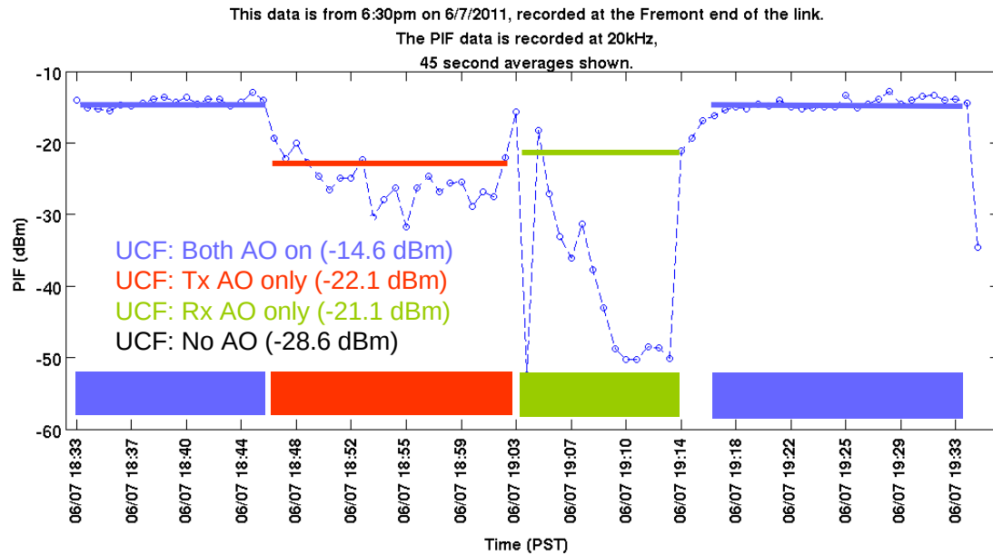
Figure 16 (a) PIB data taken during 6:30-7:30 pm on June 7 at the Fremont end of the path and (b) PIF data taken at the Fremont end of the path during the same time.
