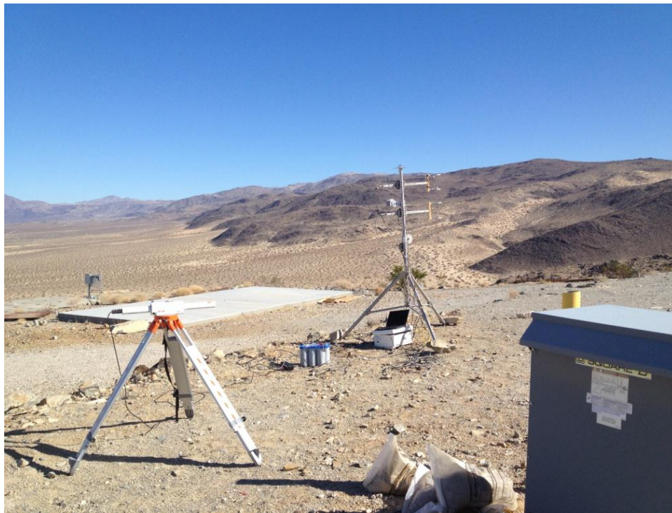
Figure 24 UCF weather station and SLS-20 transmitter.
