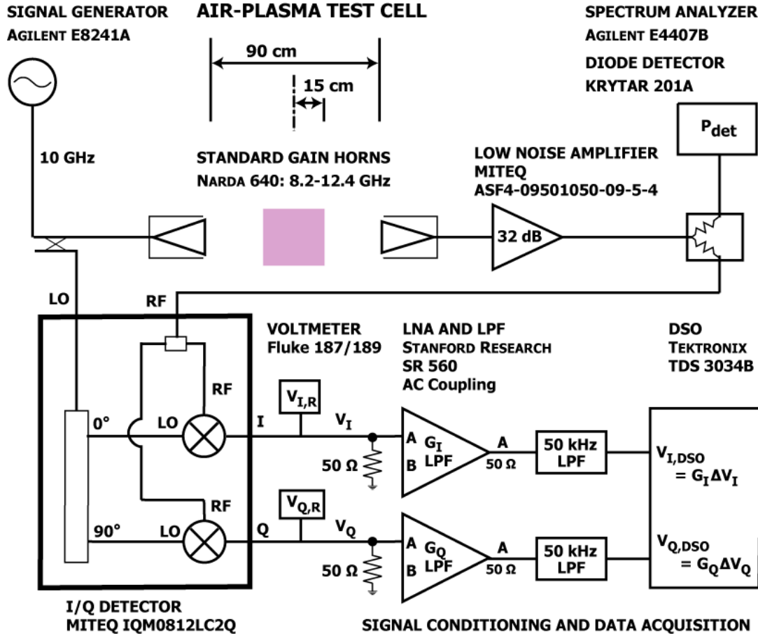
Figure 4. I/Q detection system overview.
