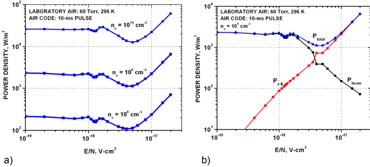
Figure 11. Theoretical curves of power required to generate and sustain plasma as a function of E/N at 60 Torr. a) Total power vs E/N. b) Total power, beam power, and \mathbf{J} \cdot \mathbf{E} vs E/N.
