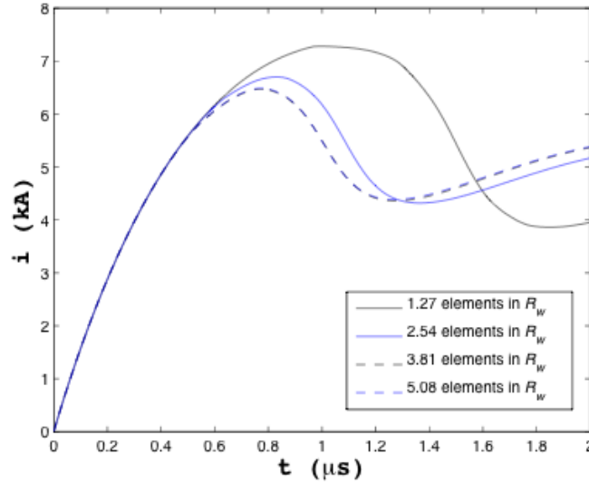
Figure 5. Current as a function of time for several mesh resolutions, at 400 R_w .
