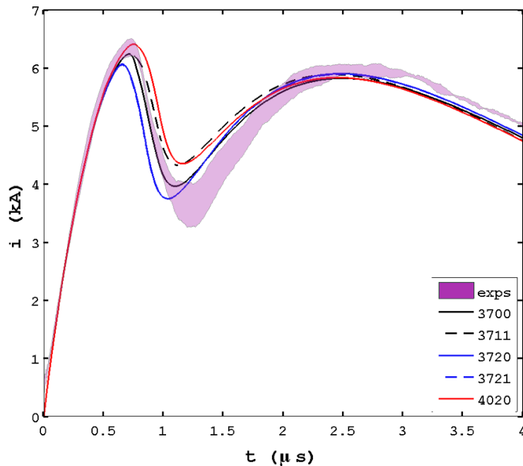
Figure 16. Current as a function of time for experiments and simulations using the Al EOS models 3700, 3711, 3720, 3721 and the Al 2024 alloy model, 4020.
