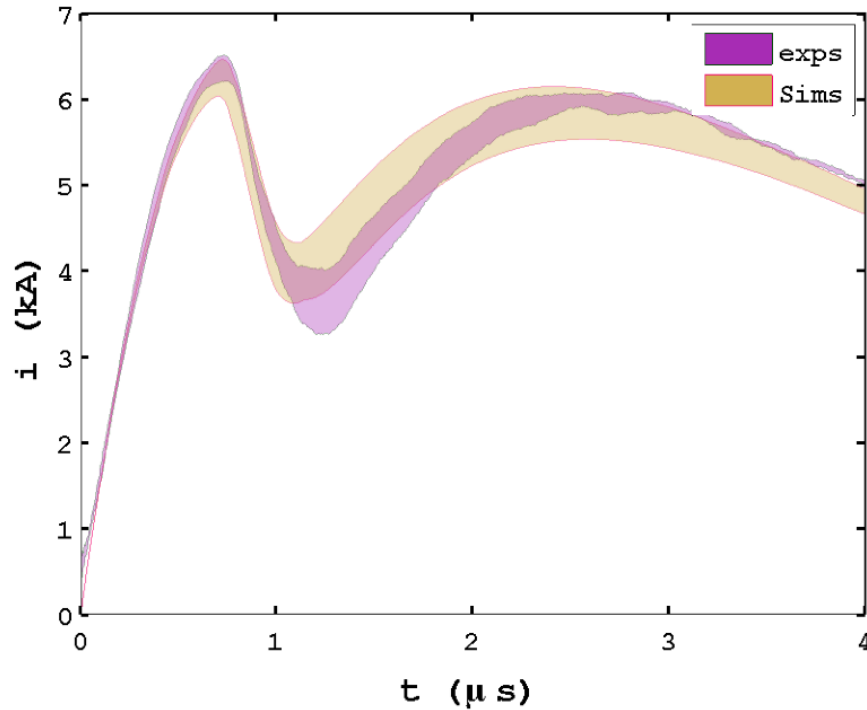
Figure 19. Current as a function of time for experiments and simulations using the Al EOS 3700 and pure Al EC, with quantified uncertainty.
