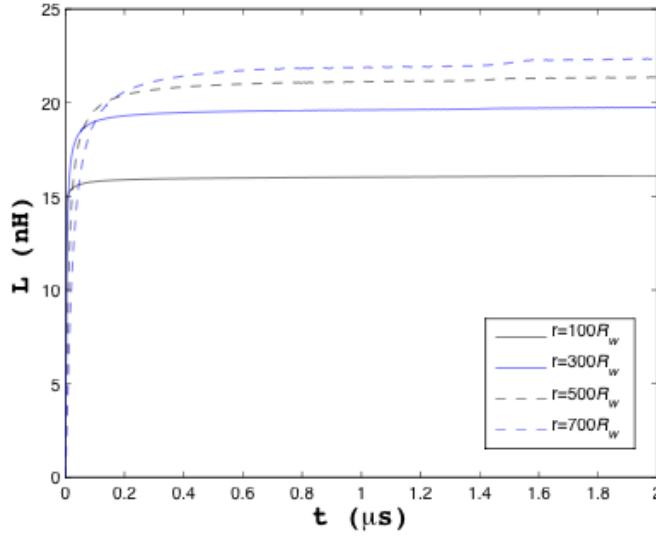
Figure 3. Load inductance as a function of time for low-voltage simulations.
