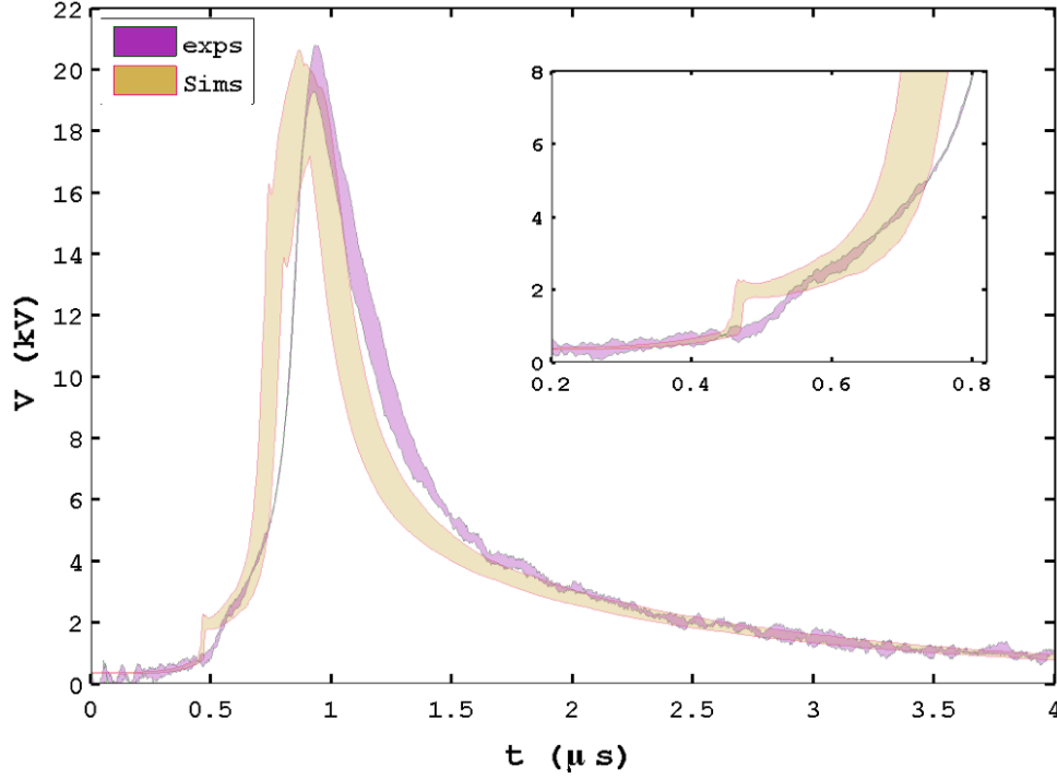
Figure 20. Voltage as a function of time for experiments and simulations using the Al EOS 3700 and pure-Al EC, with quantified uncertainty.
