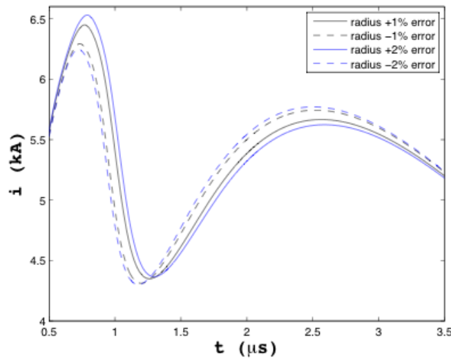
Figure 12. Effect of wire diameter measurement error.
