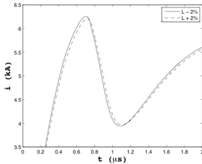
Figure 10. Current as a function of time for a sample simulation with a \pm 2\% error in the external inductance.
