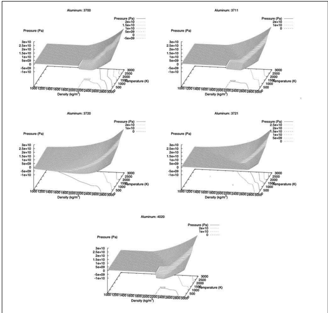
Figure B-1. EOS surfaces p(\rho, T) from SESAME and ANEOS data in ALEGRA repository.
