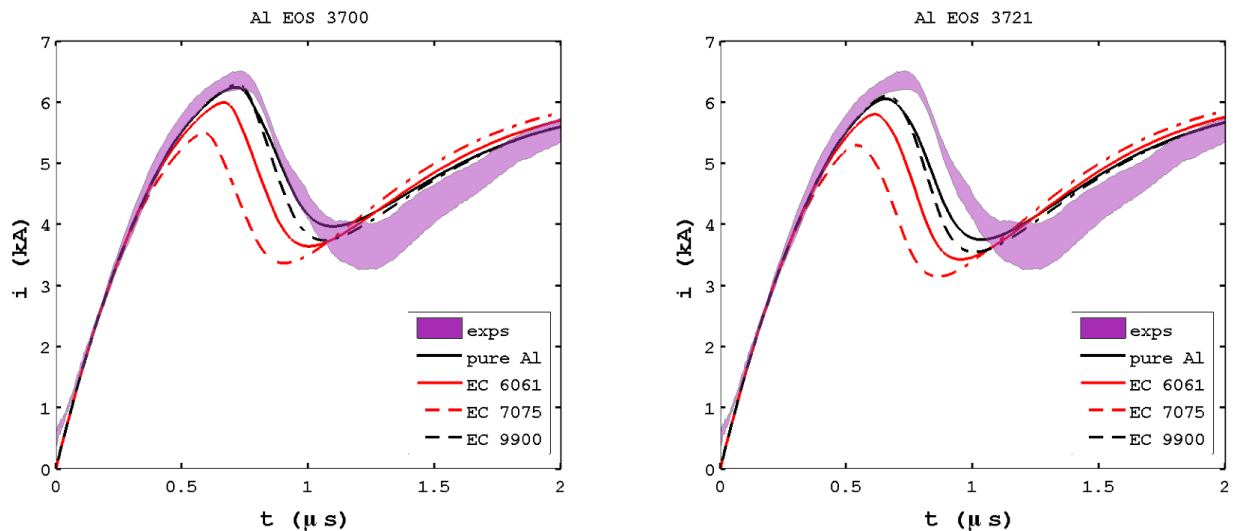
Figure 18. Current as a function of time for experiments and simulations using the Al EOS 3700 (left) and 3721 (right) with pure Al, 6061, 7075, and 9900 conductivity models.
