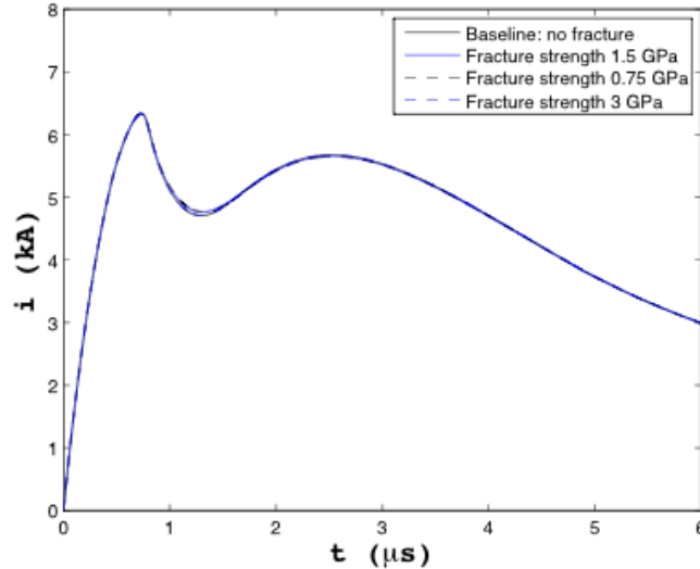
Figure 8. Role of fracture in the current trace for simulation with density perturbation.
