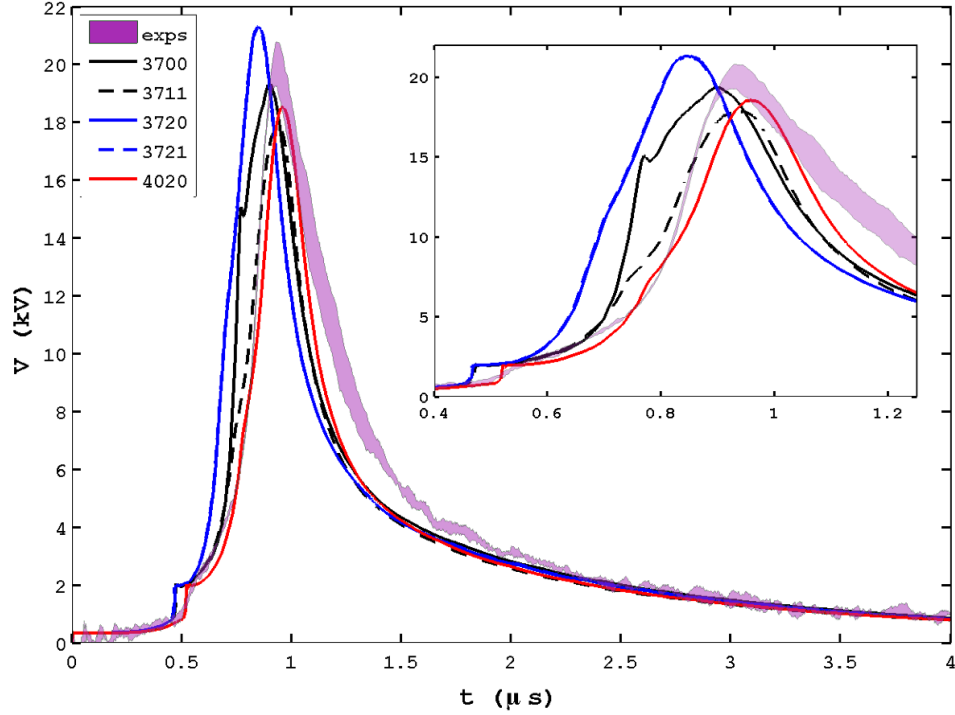
Figure 17. Voltage as a function of time for experiments and simulations using the Al EOS 3700, 3711, 3720, 3721 and the Al 6061 alloy, 4020.
