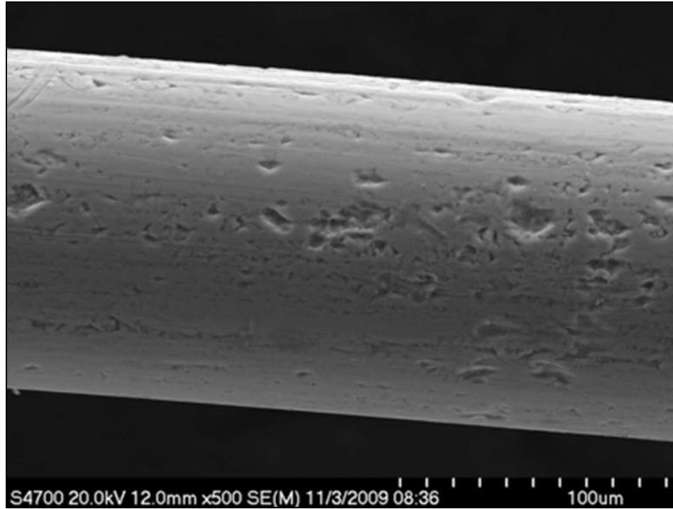
Figure 1. SEM image of an Al wire used in this study.
