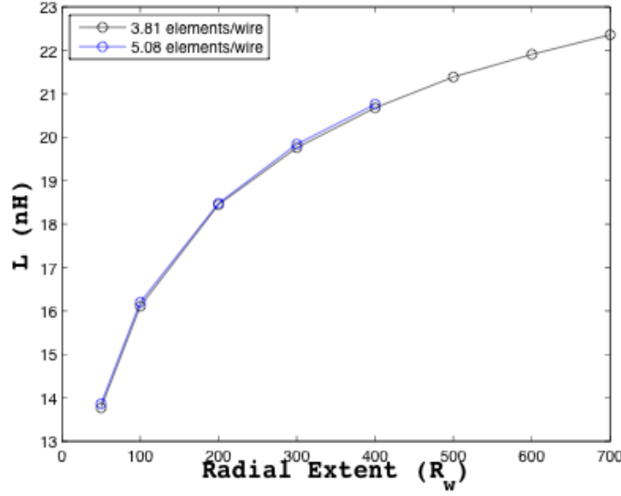
Figure 4. Load inductance as a function of radial mesh extent for low-voltage simulations.
