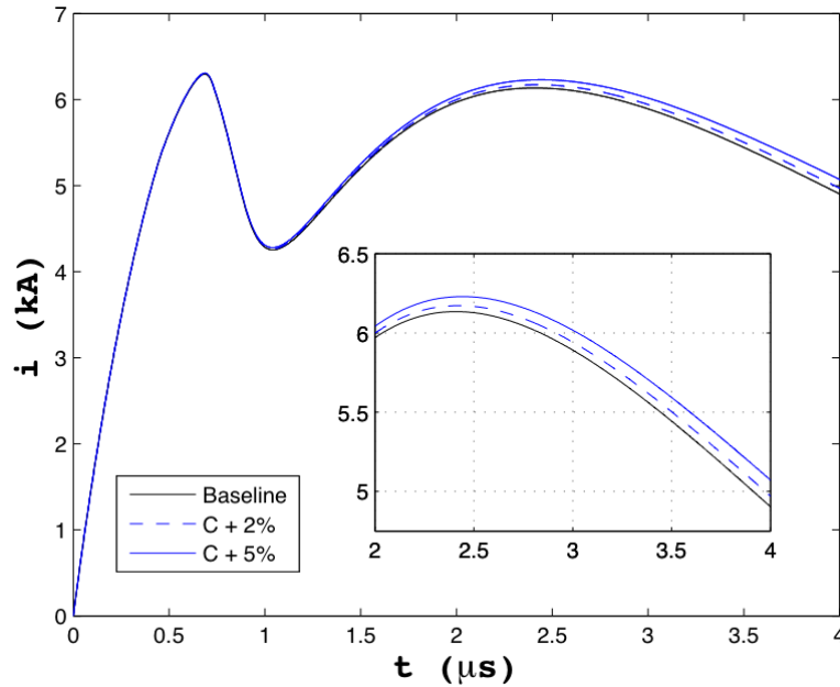
Figure 21. Current as a function of time for baseline calculations and uncertainty in the external capacitance.
