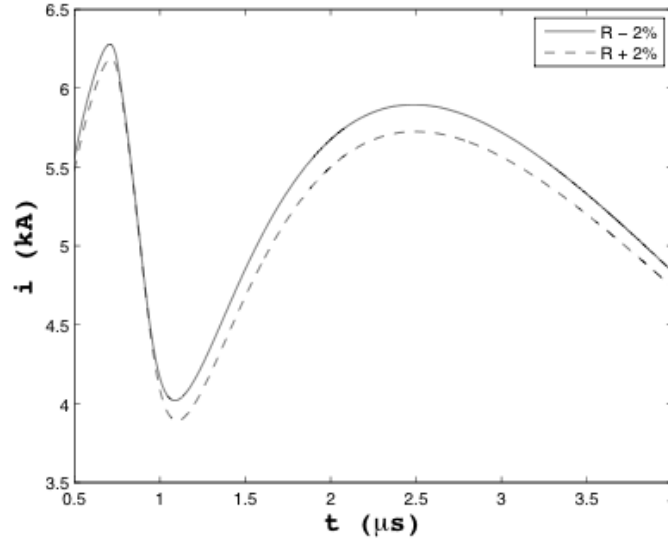
Figure 11. Current as a function of time for a sample simulation with a \pm 2\% error in the resistance.
