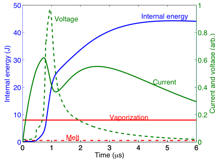
Figure 6. Normalized histories of current and voltage for the present EW system, with wire internal energy. Horizontal red lines indicate estimated energies for phase changes.
