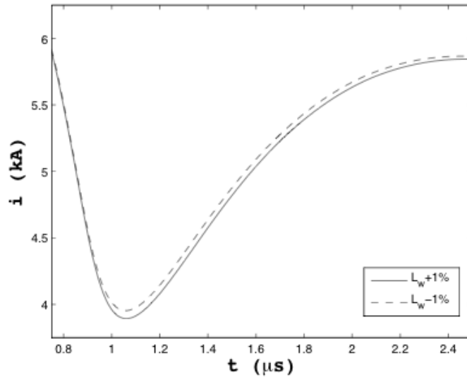
Figure 13. Effect of wire length measurement error (subregion of the current trace).
