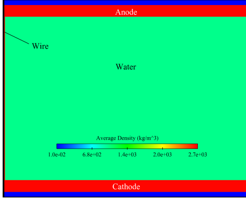
Figure 2. Full domain, half symmetry of the initial state of a typical exploding wire simulation setup.
