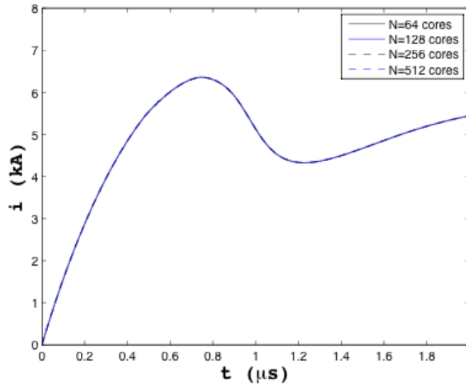
Figure 7. Current as a function of time for a sample simulation testing parallel scalability.
