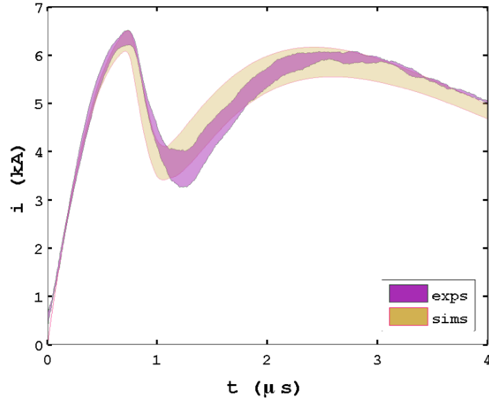
Figure C-1. Current as a function of time for experiments and simulations using the Al EOS 3700 and the LMD 9900 EC model, with quantified uncertainty.
