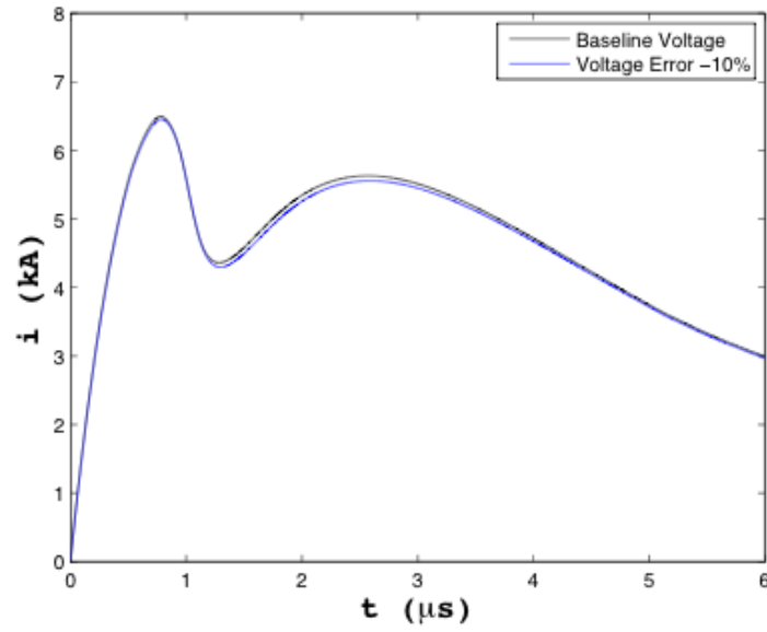
Figure 9. Current trace as a function of time for sample simulation and maximum error of 10% in voltage.
