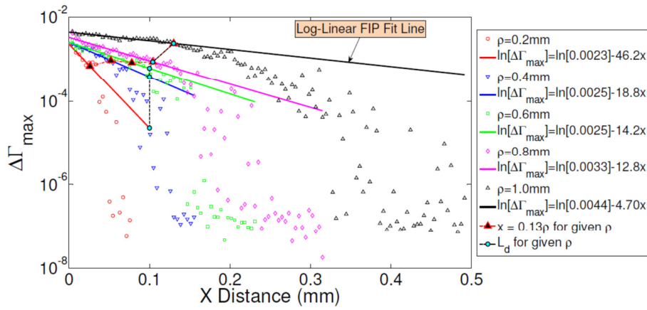
(c) FIP distribution as a function of X-distance from notch root.
