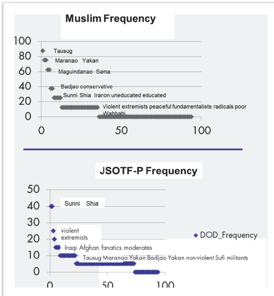
Figure 4. Comparison of free-list task responses between JSOTF-P members and Muslim Filipinos. Vertical scale is frequency (percent of responses); horizontal scale is item.
