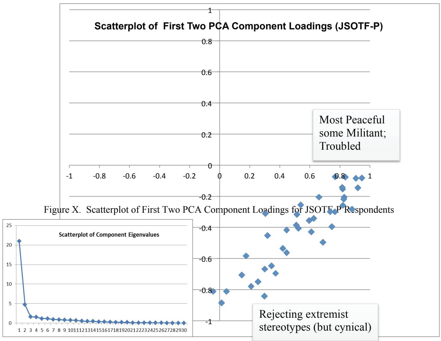
Figure 7. Scatterplot of First Two PCA Component Loadings for JSOTF-P Respondent
