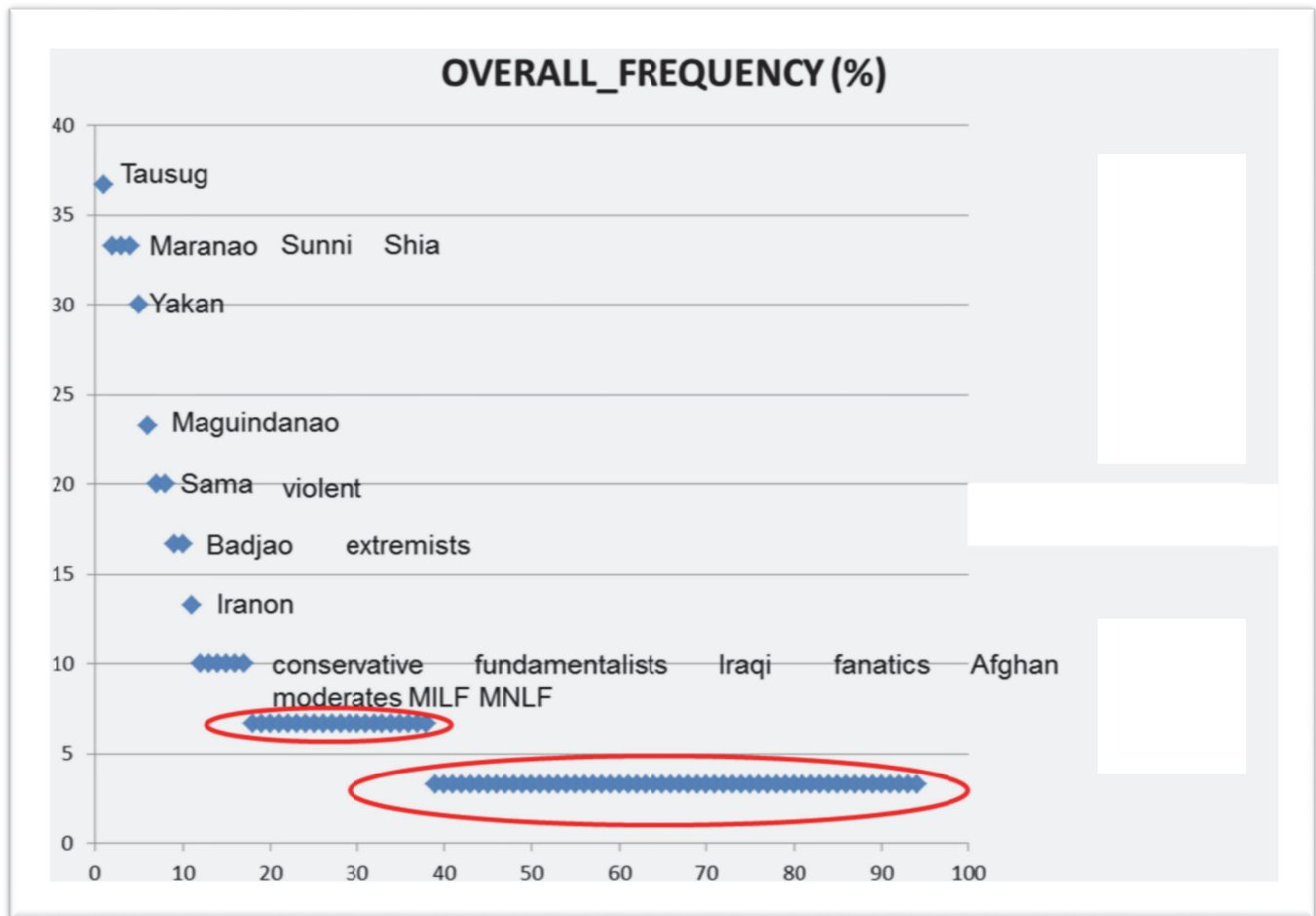
Figure 3. Raw frequencies of items from free-list task. The items mentioned infrequently (by one or two persons only) are circled in red and presented in Table 2. Vertical scale is frequency of item (percent of responses) horizontal scale is domain item. (There are 97 items)
