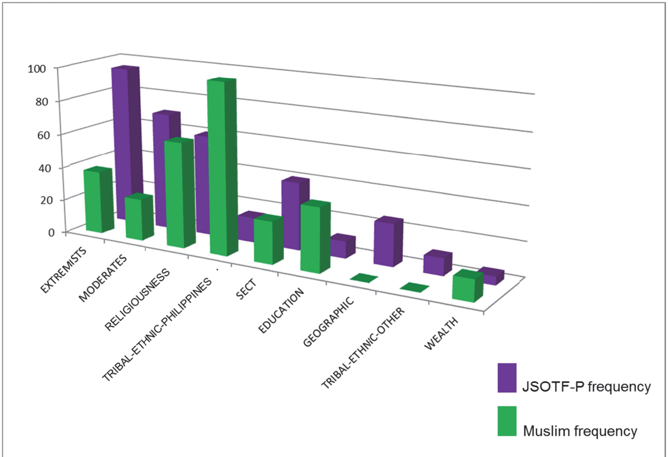
Figure 5. Free-list responses binned into categories. (Vertical scale is percent of responses)
