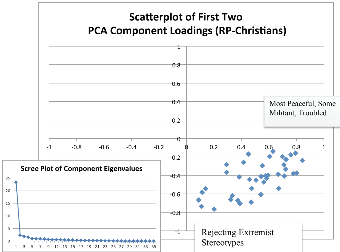
Figure 8. Scatterplot of First Two PCA Component Loadings for Philippine Christian Respondents
